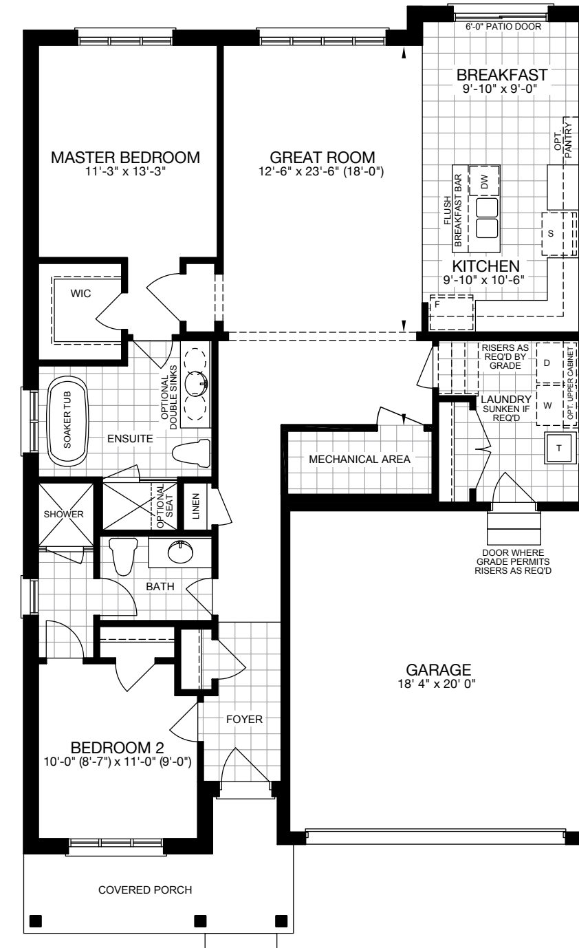
FIRST FLOOR PLAN EL-A
