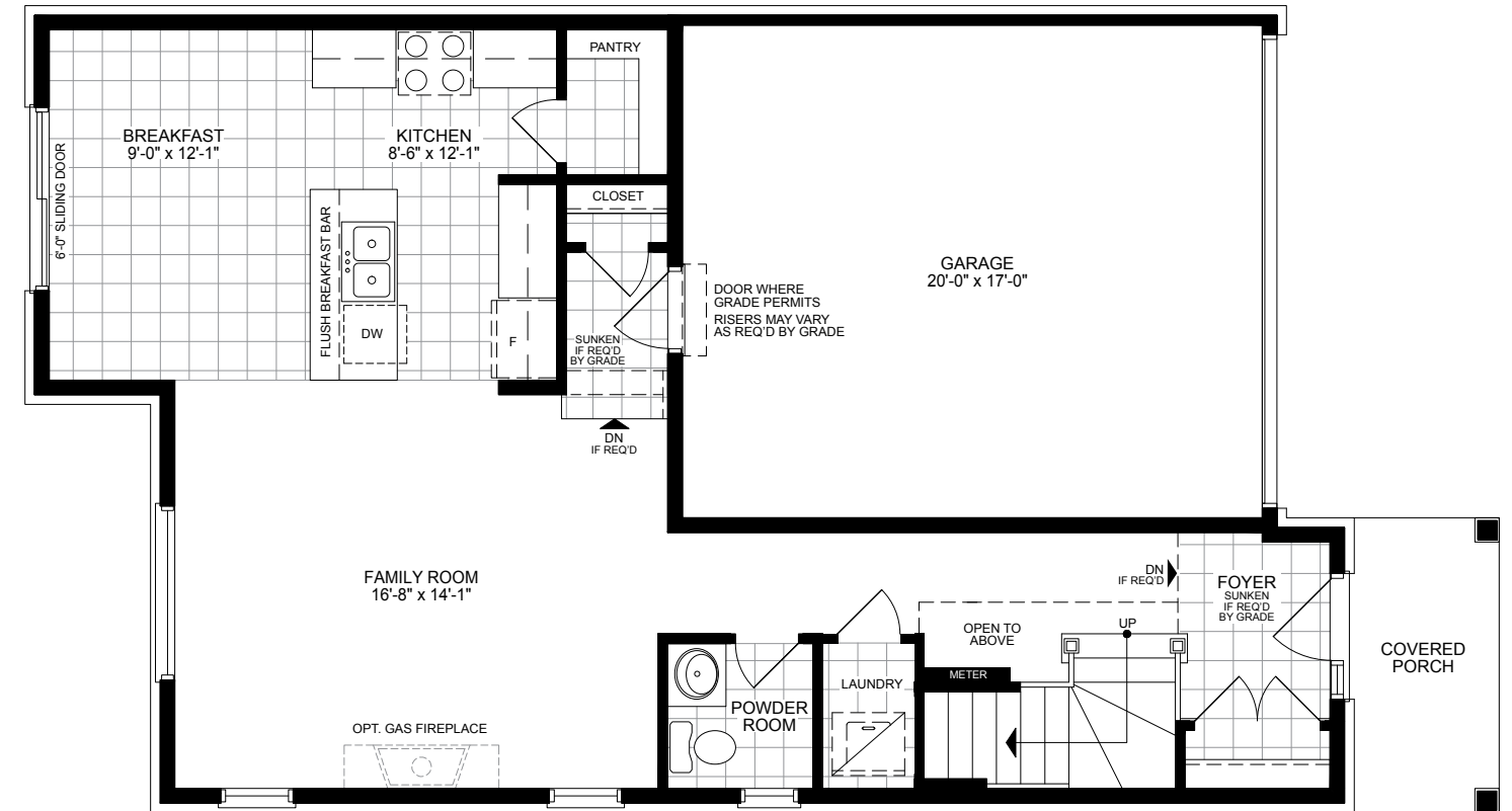
FIRST FLOOR PLAN EL-A & B
