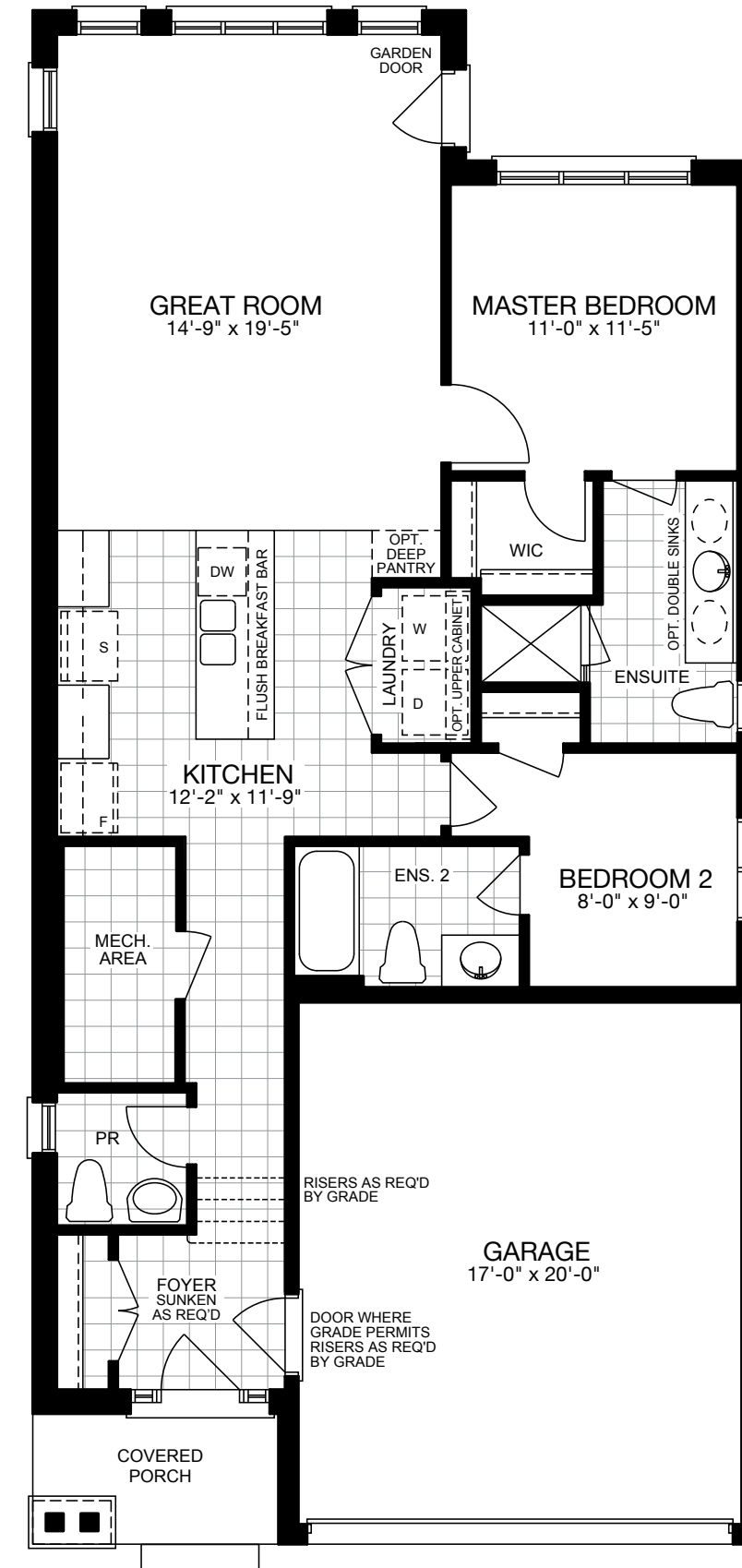
FIRST FLOOR PLAN EL-A
