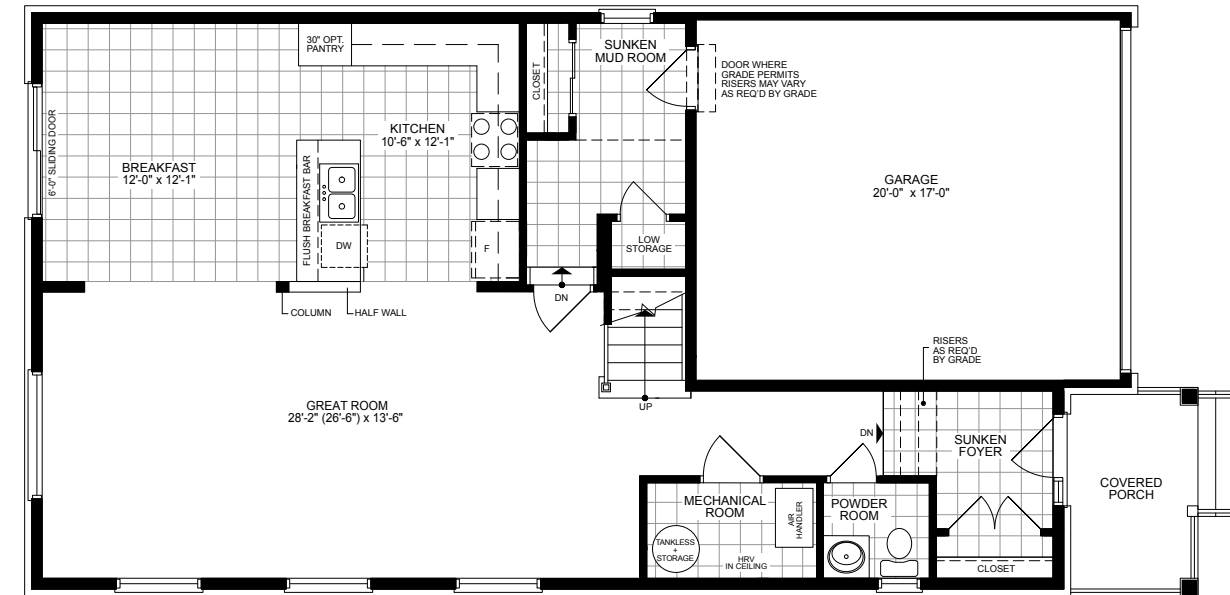
FIRST FLOOR PLAN EL-A
