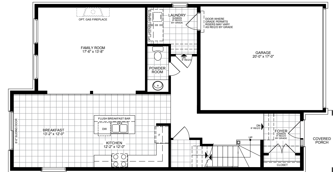
FIRST FLOOR PLAN EL-A
