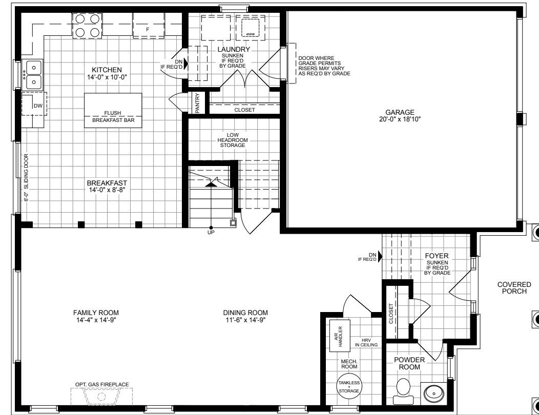
FIRST FLOOR PLAN EL-A & B
