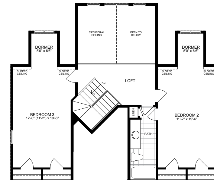
LOFT FLOOR PLAN EL-A & B
