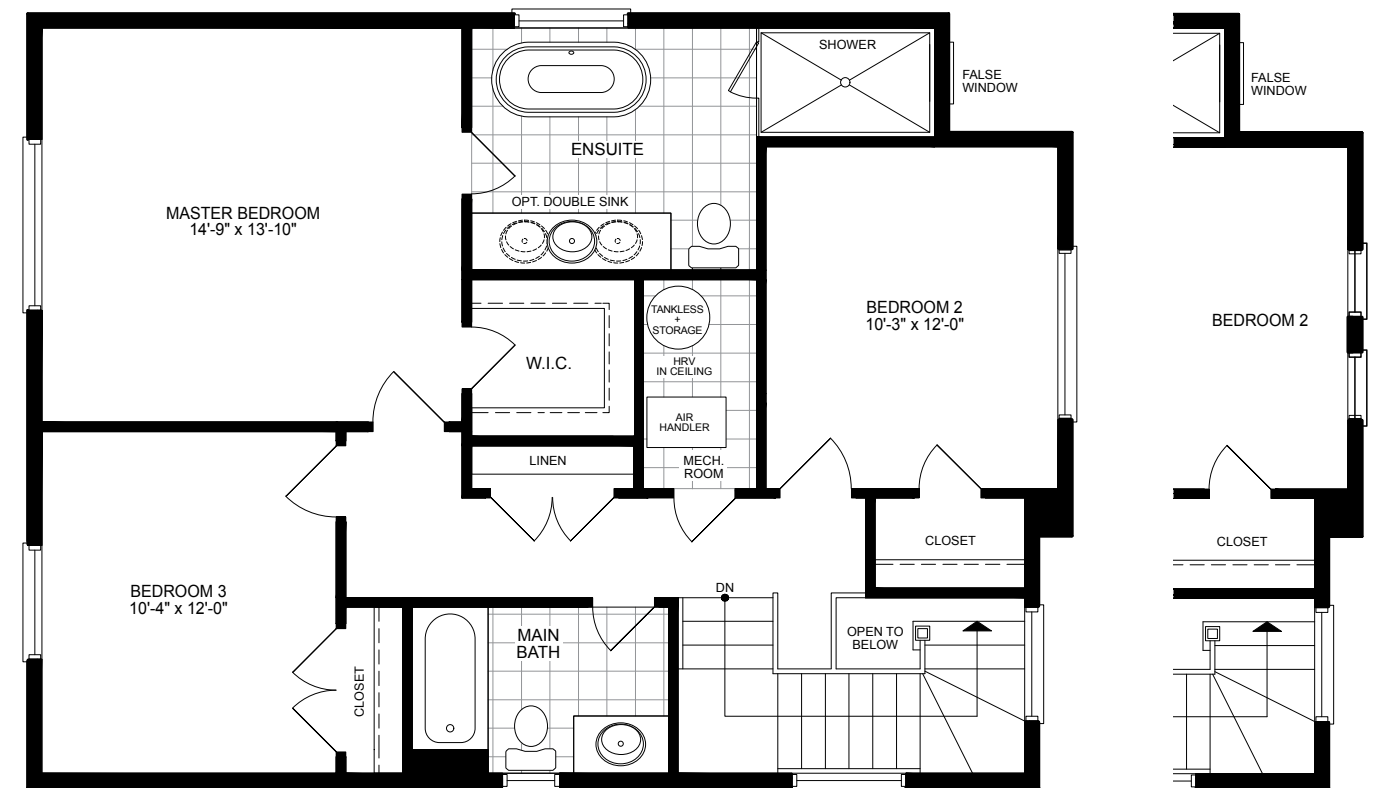
SECOND FLOOR PLAN EL-A
