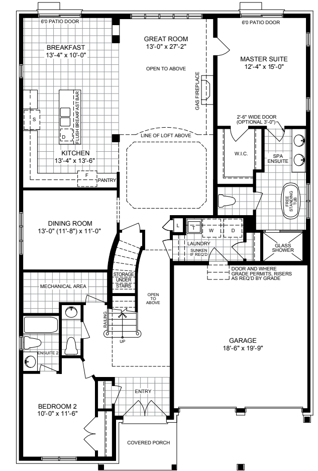
OPTIONAL FIRST FLOOR PLAN EL-A
