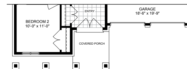
PARTIAL FIRST FLOOR PLAN EL-B
