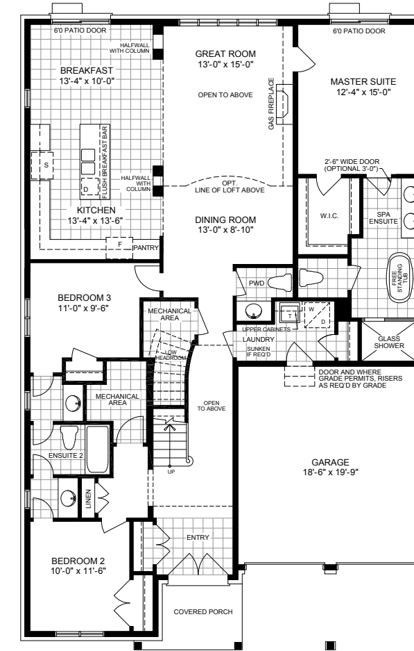
FIRST FLOOR PLAN EL-A
