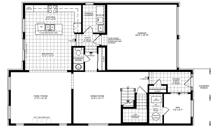
FIRST FLOOR PLAN EL-A & B
