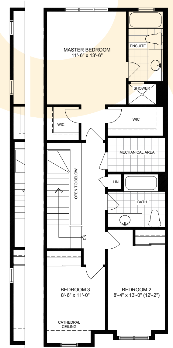
PARTIAL SECOND FLOOR PLAN EL-A & B END SECOND FLOOR PLAN EL-A & B
