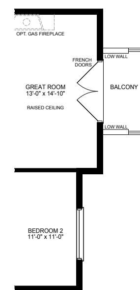
PARTIAL SECOND FLOOR PLAN EL-B
