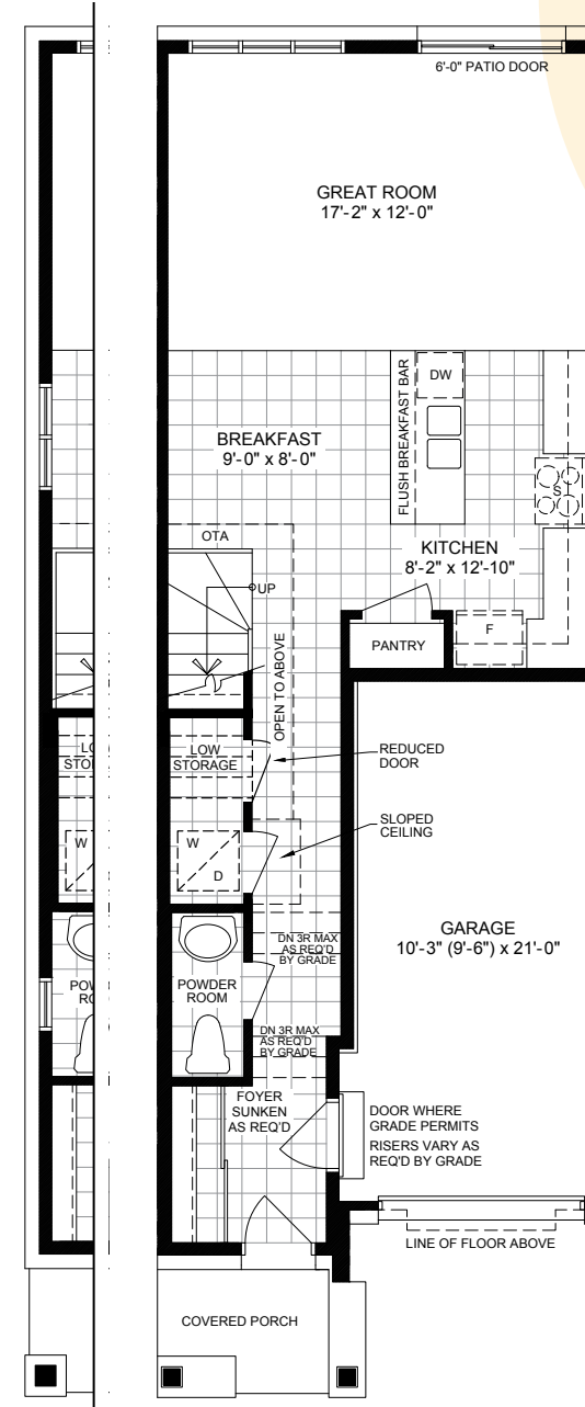
PARTIAL FIRST FLOOR PLAN EL-A & B END FIRST FLOOR PLAN EL-A & B
