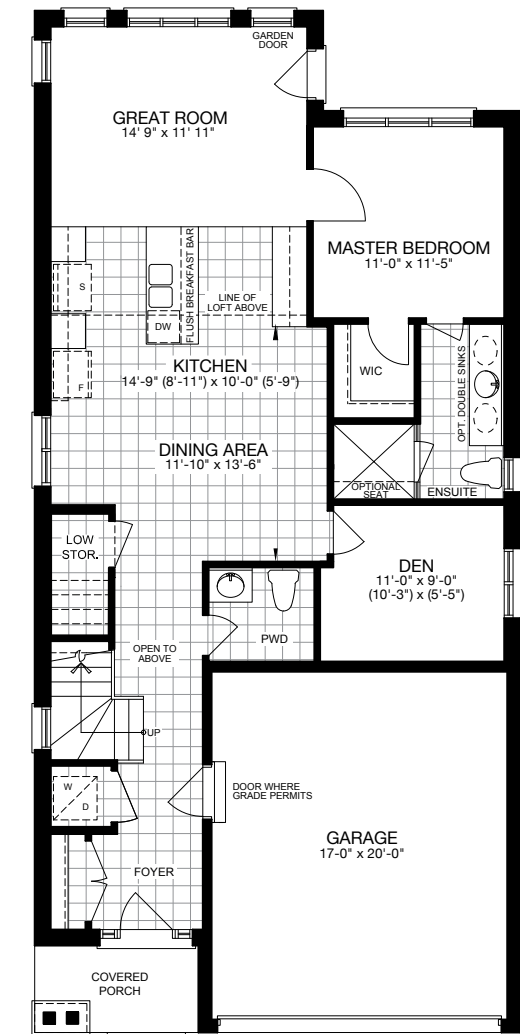
OPTIONAL FIRST FLOOR PLAN EL-A
