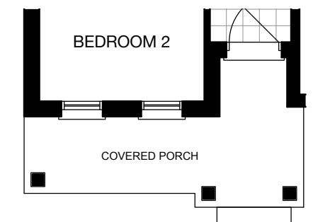
PARTIAL FIRST FLOOR PLAN EL-B
