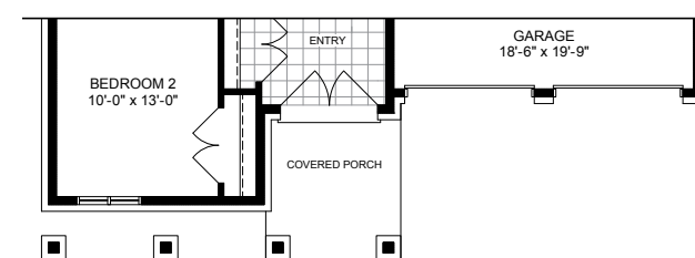
OPTIONAL FIRST FLOOR PLAN EL-B
