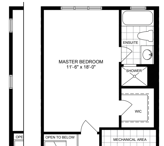
PARTIAL SECOND FLOOR PLAN OPTIONAL BEDROOM EL-A & B END PARTIAL SECOND FLOOR PLAN OPTIONAL BEDROOM EL-A & B
