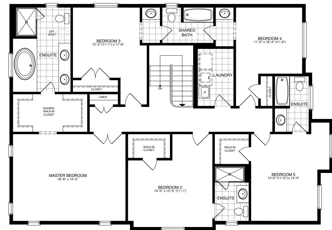
SECOND FLOOR PLAN EL-A & B
