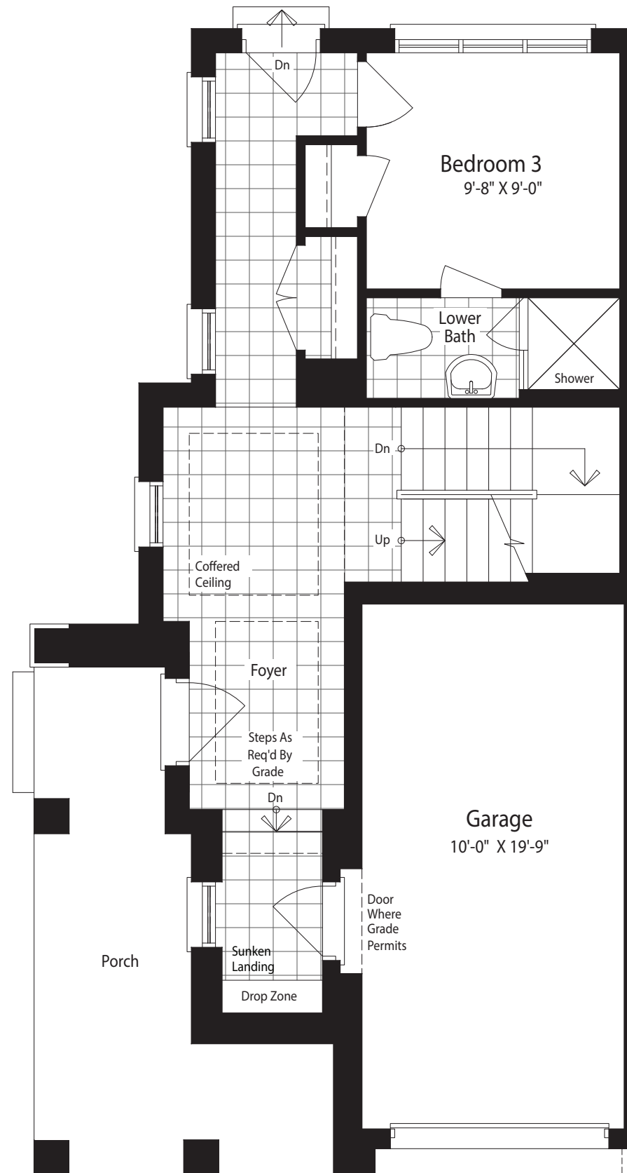
Ground Floor Plan Elevation 'B'
