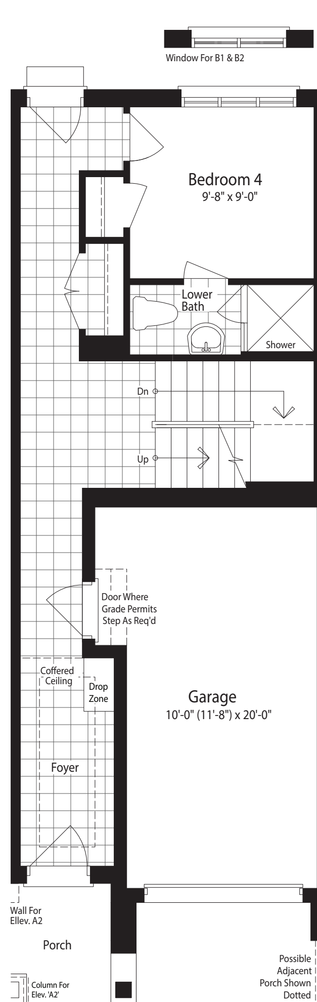
Ground Floor Plan Elevation 'A1' & 'A2'
