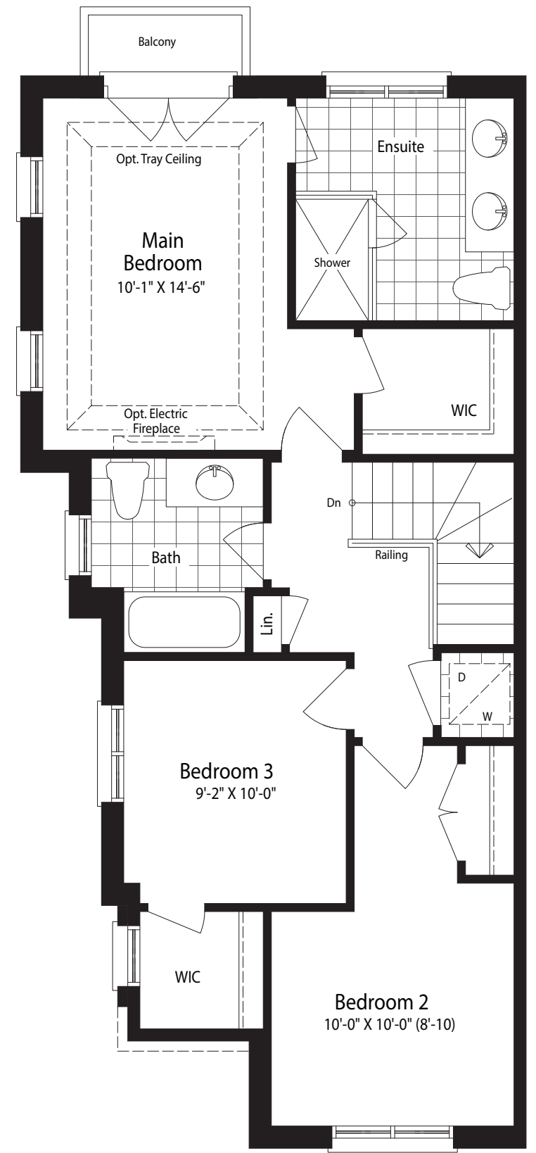
Upper Floor Plan Elevation 'A'
