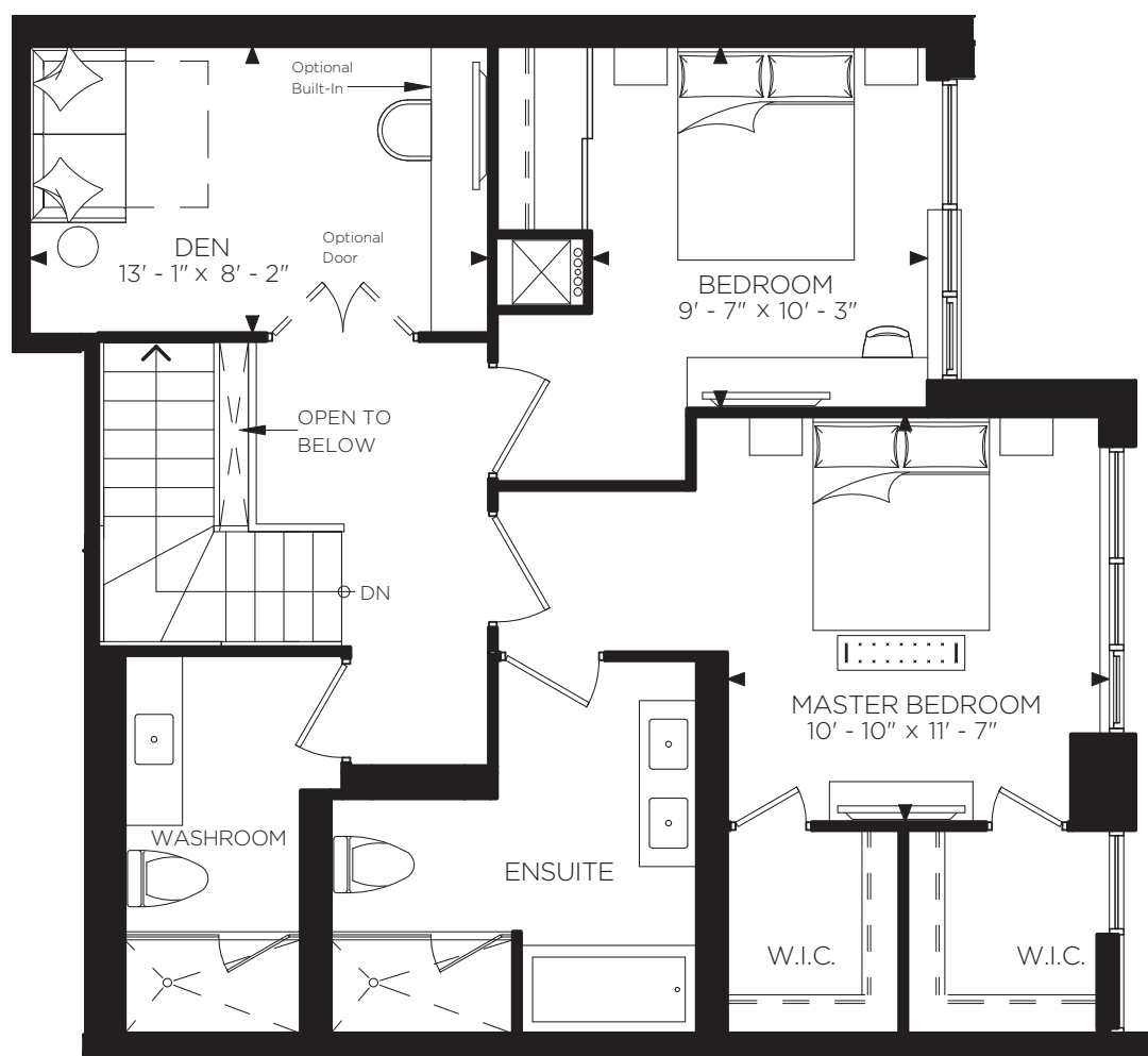
LEVEL 2
