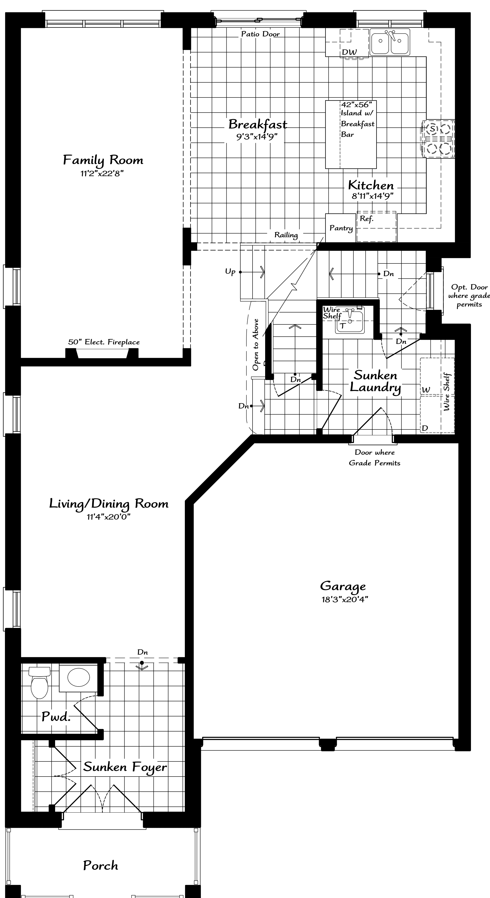
First Floor Plan 'A'/'B'/'C'
