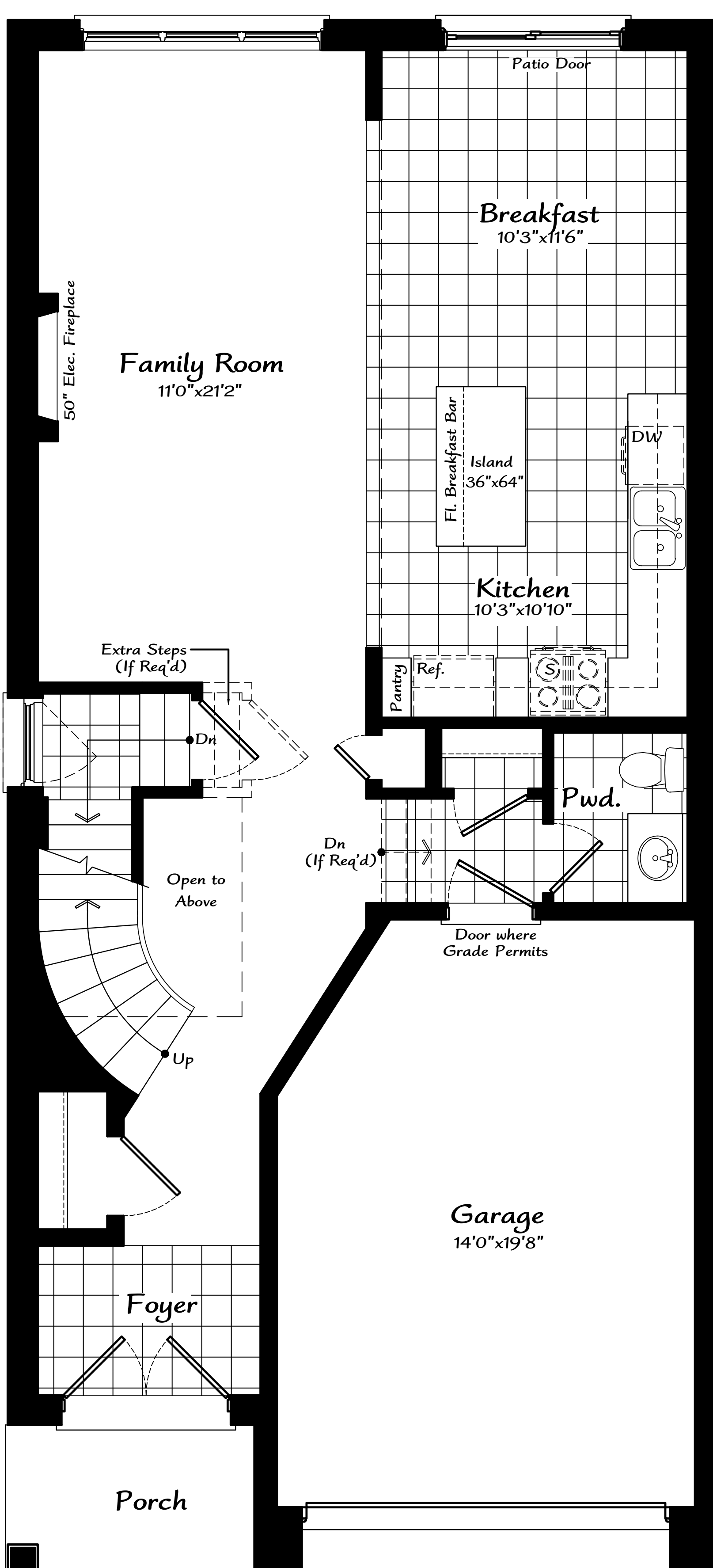
First Floor Plan 'A'
