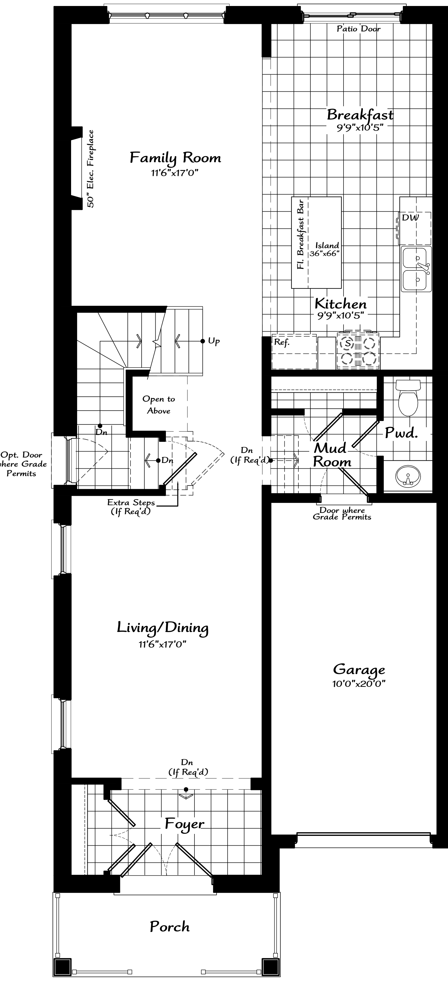
First Floor Plan 'A'/'B'/'C'
