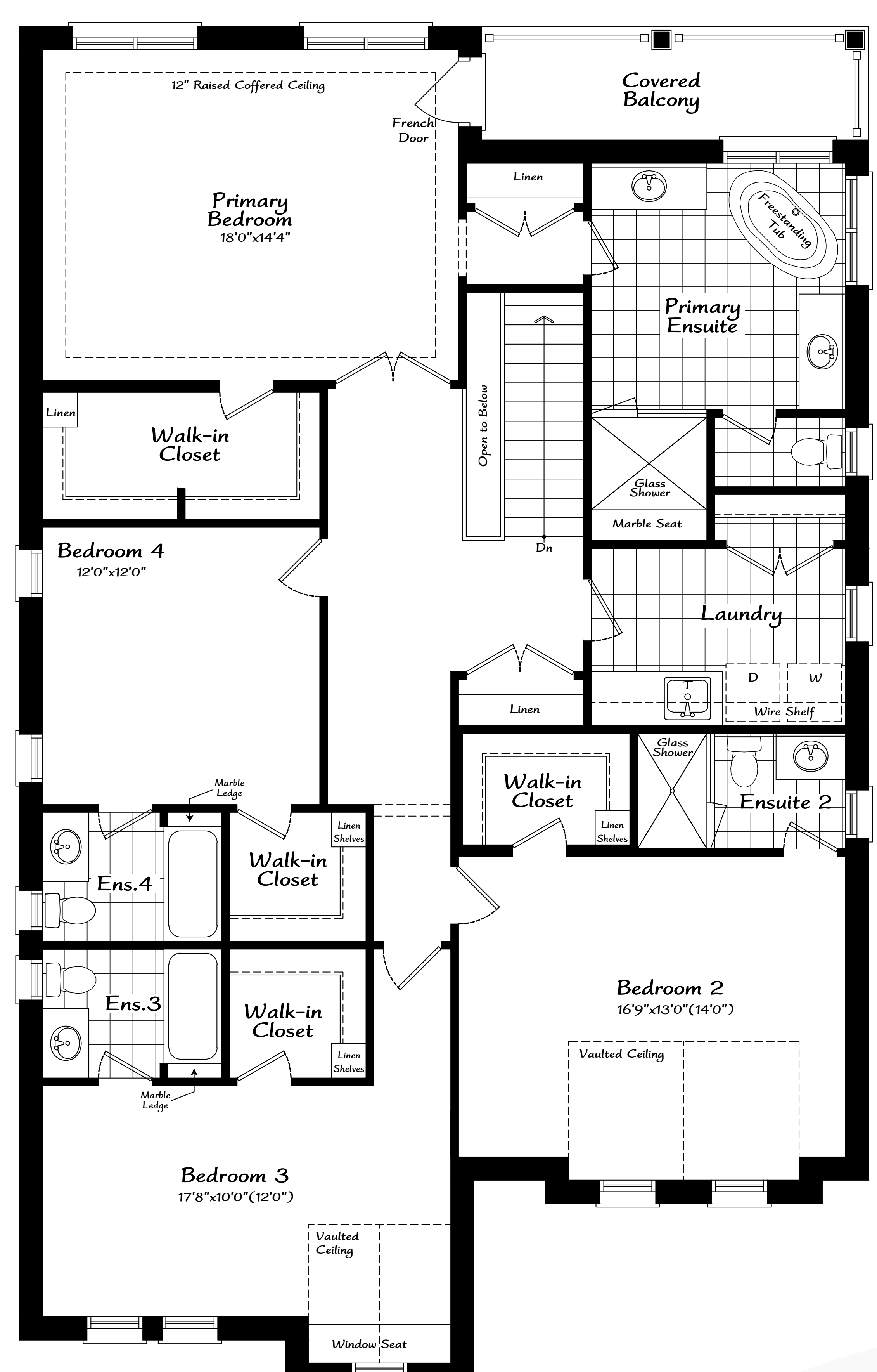
Second Floor Plan 'A'
