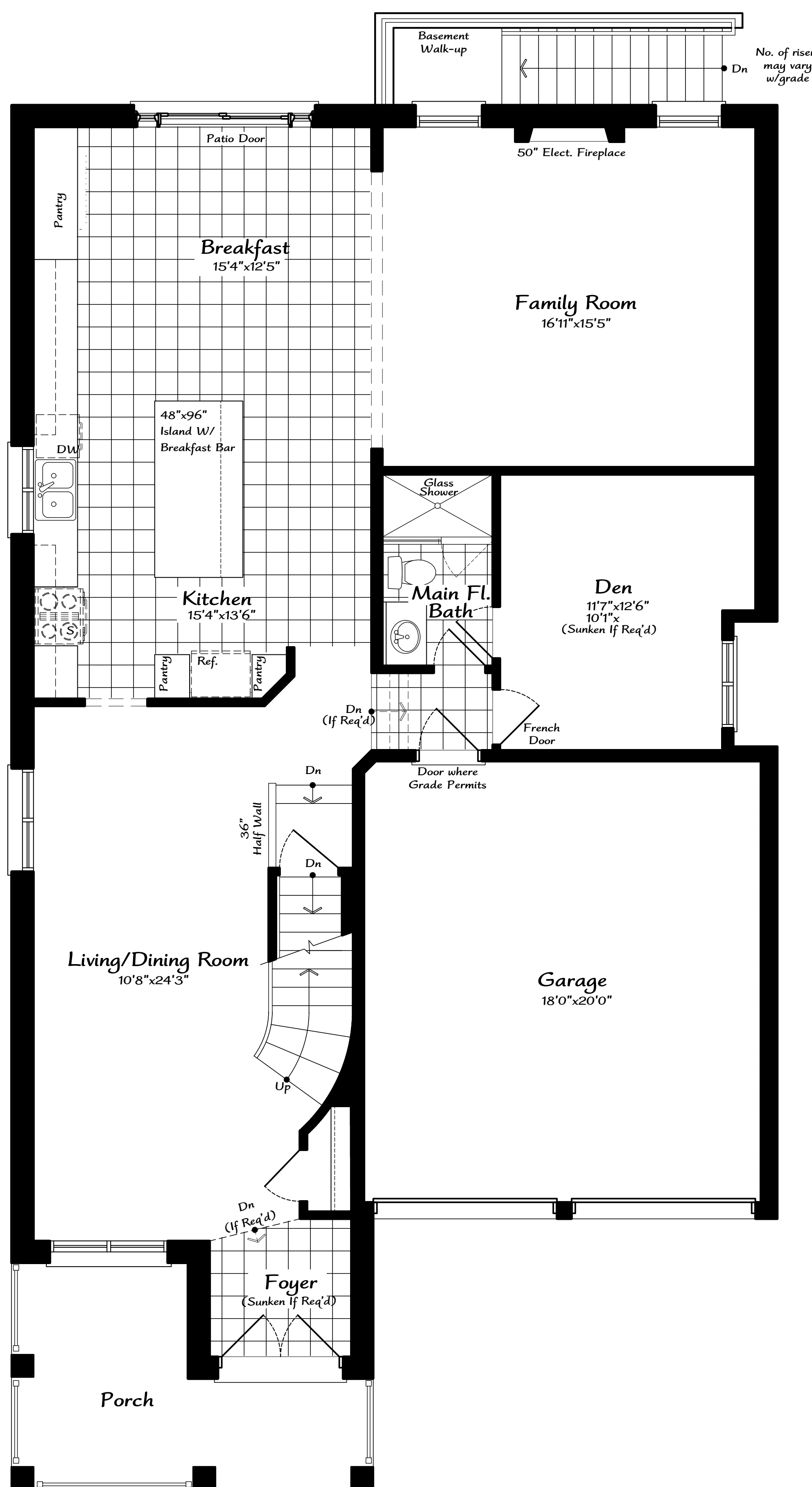
First Floor Plan 'A'/'B'
