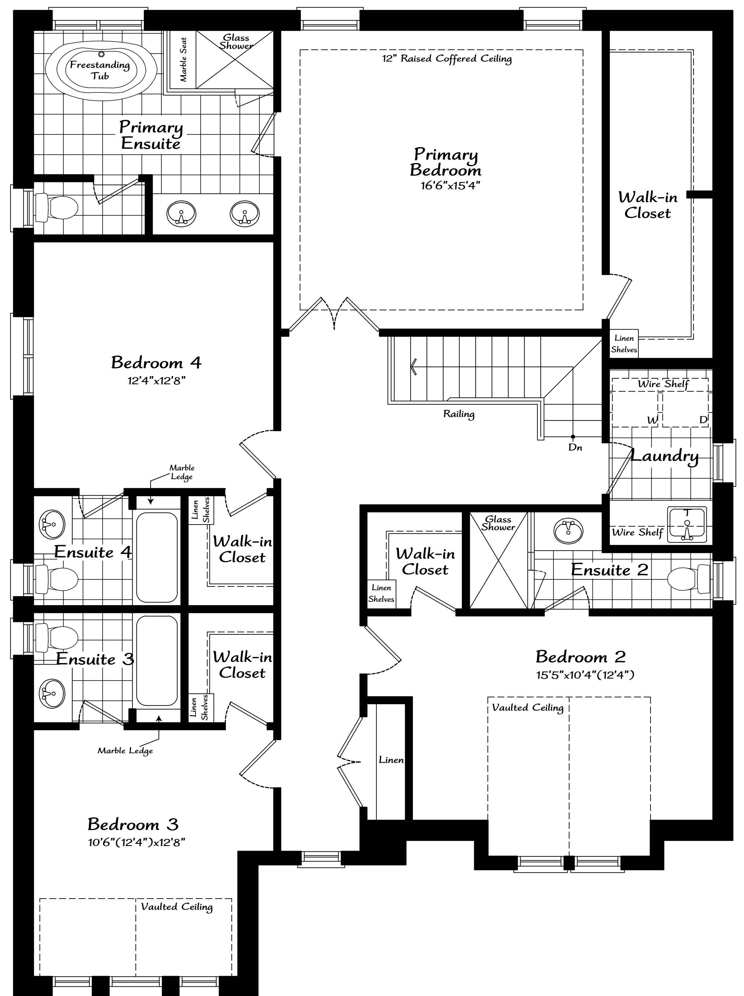
Second Floor Plan 'A'
