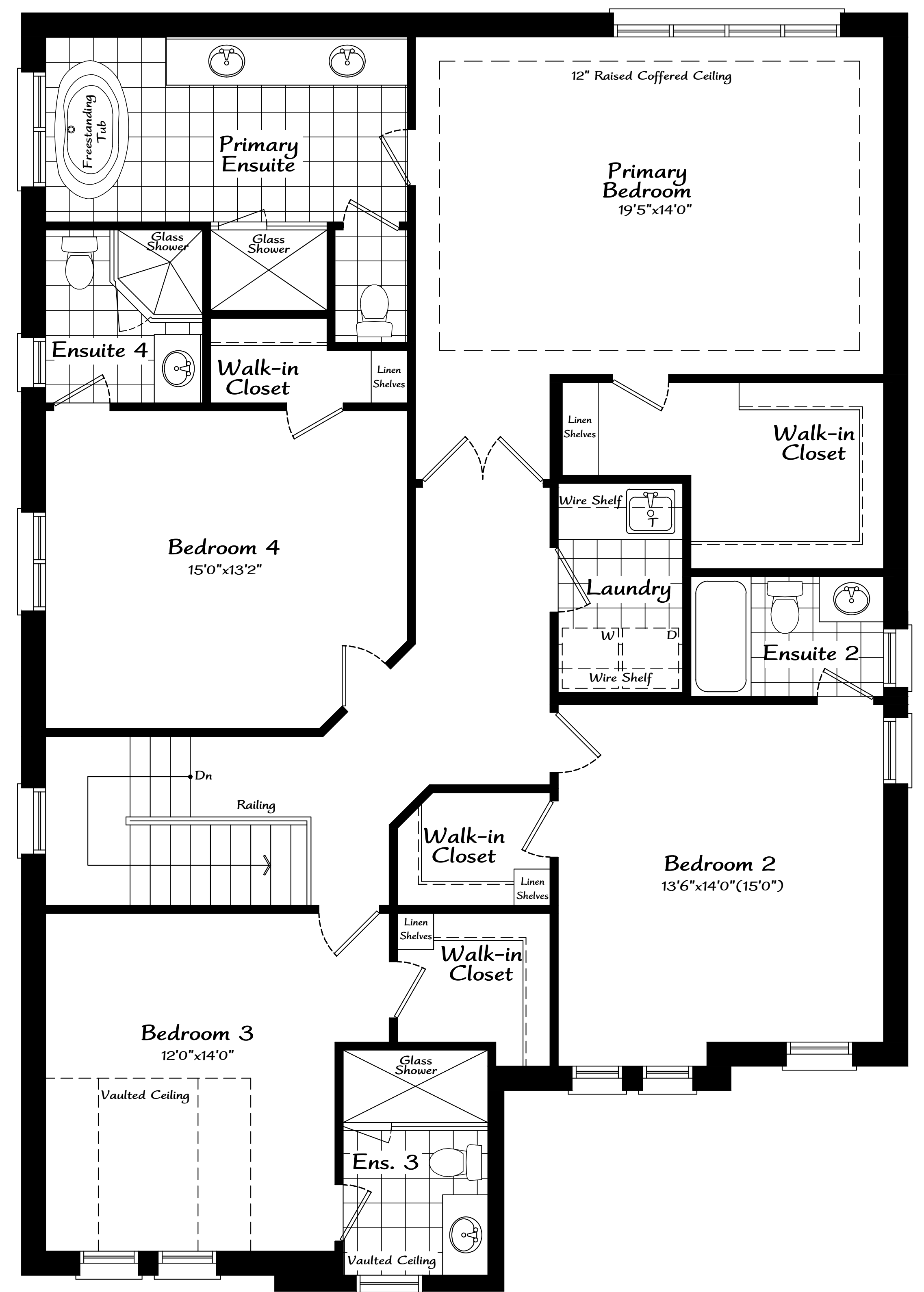
Second Floor Plan 'A'
