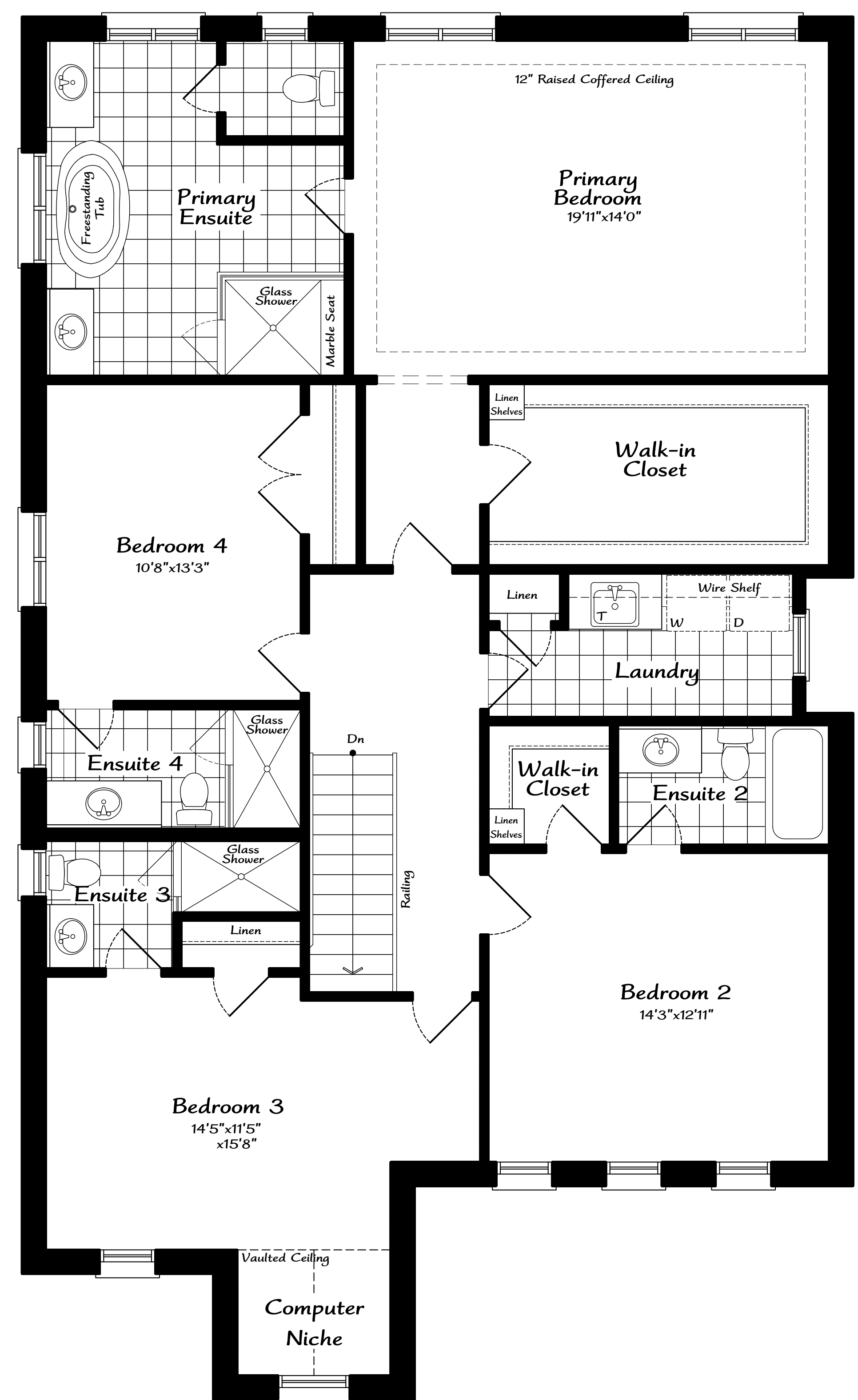
Second Floor Plan 'A'
