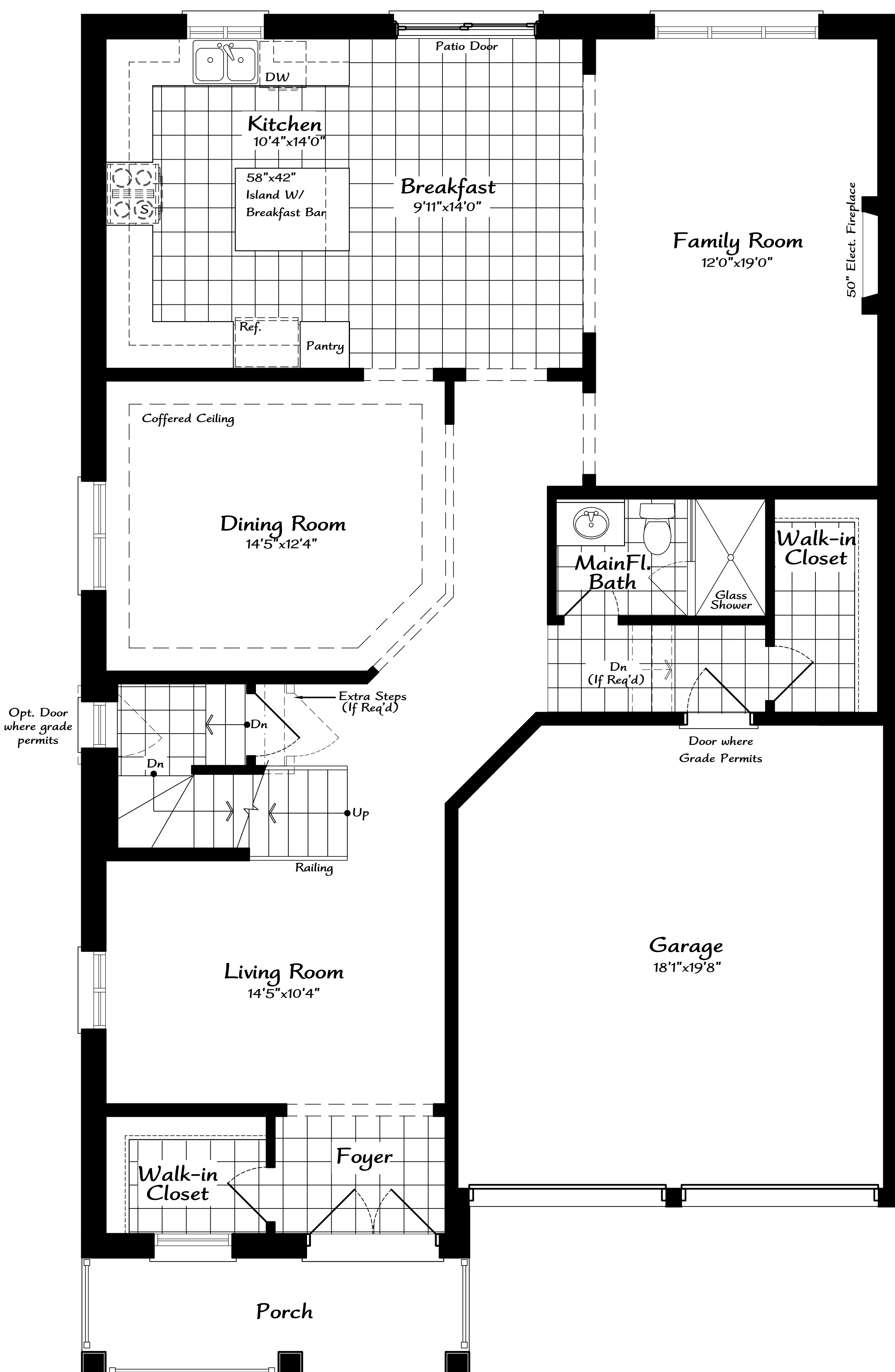
First Floor Plan 'A'
