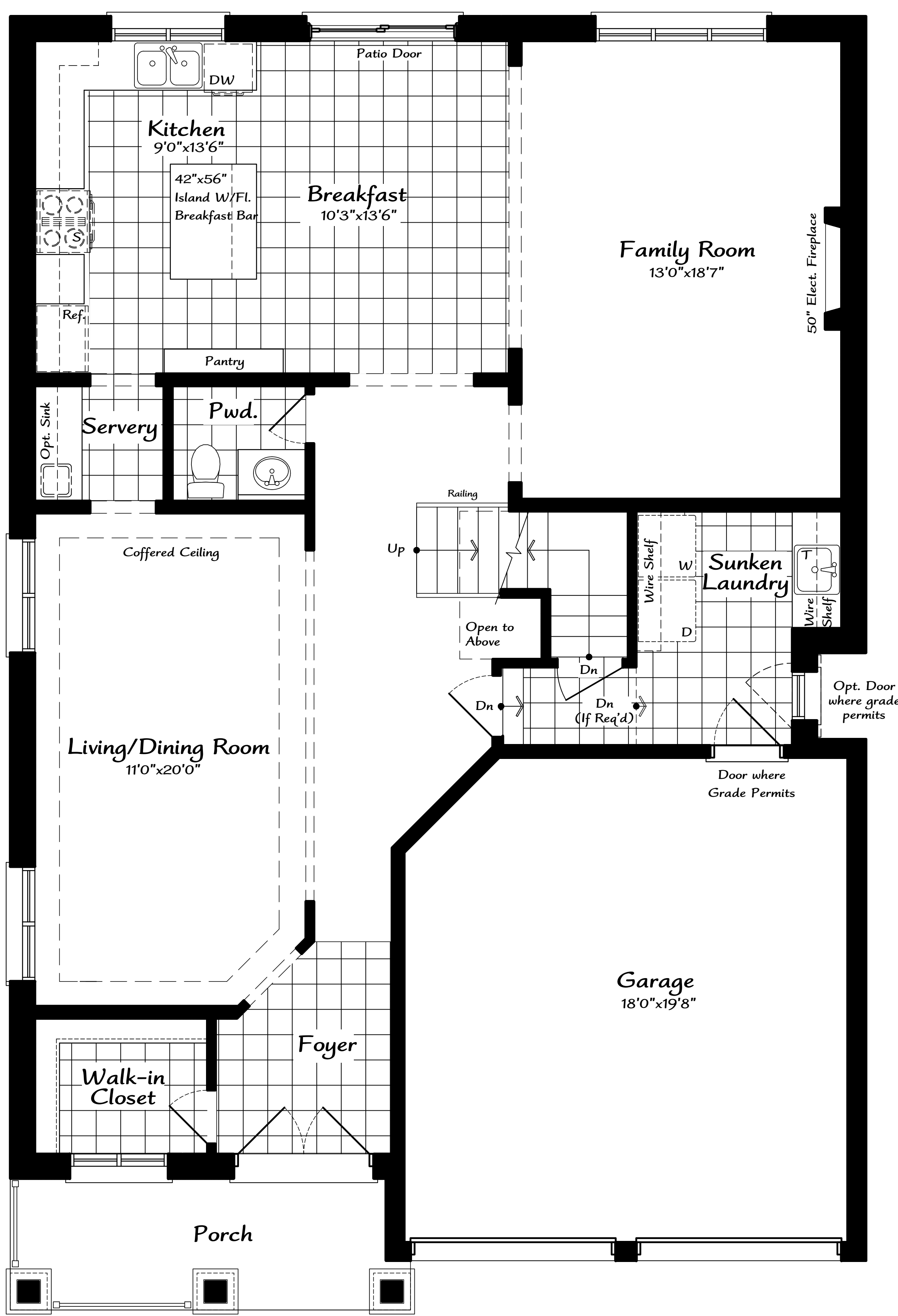
First Floor Plan 'A'
