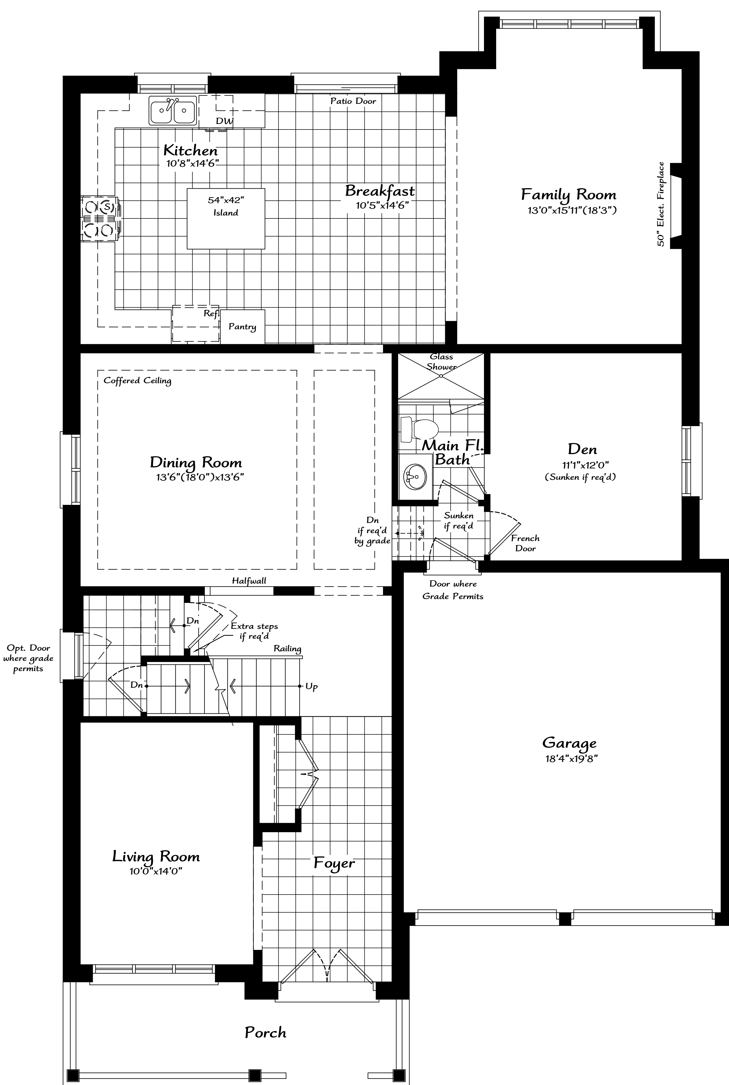
Ground Floor Plan 'A'
