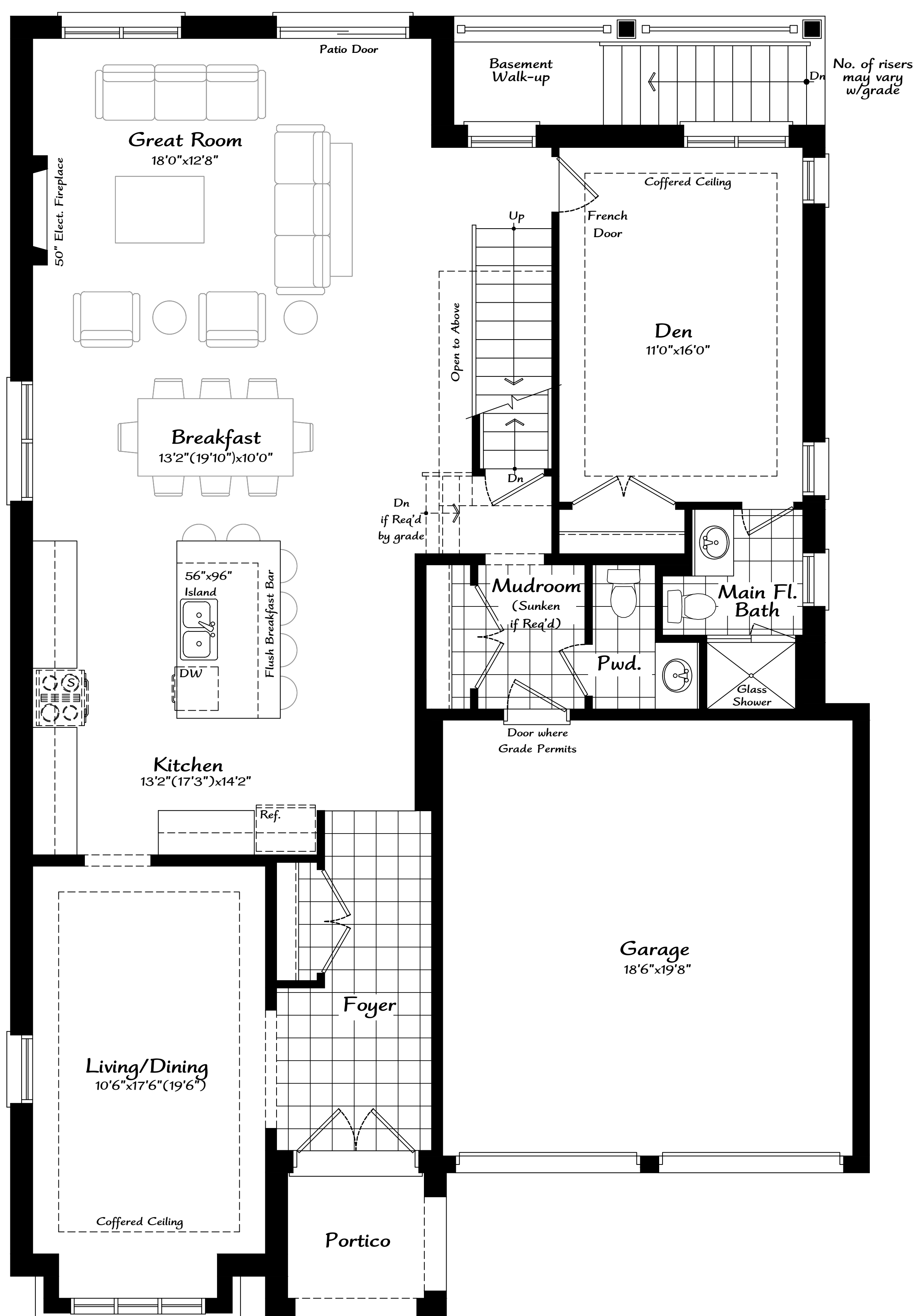
Ground Floor Plan 'A'
