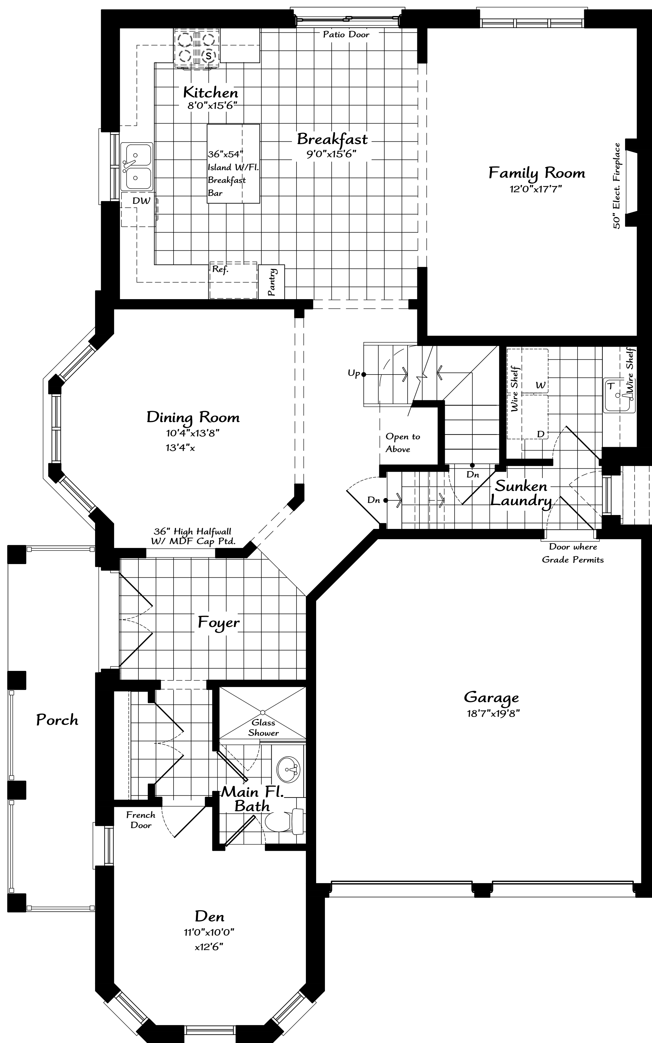
First Floor Plan 'A'
