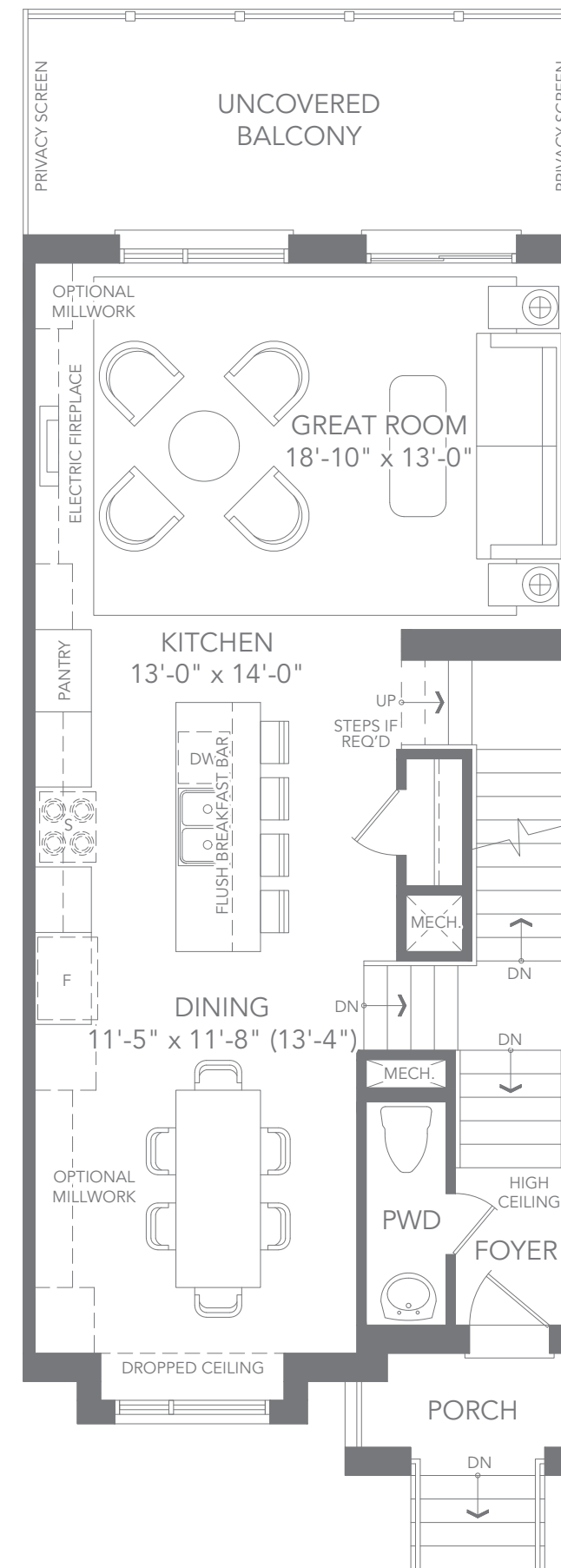
T3 INTERIOR UNIT - ELEV. C1 MAIN FLOOR PLAN
