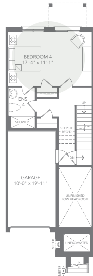
T1 INTERIOR UNIT - ELEV. A3 OPTIONAL GROUND FLOOR PLAN
