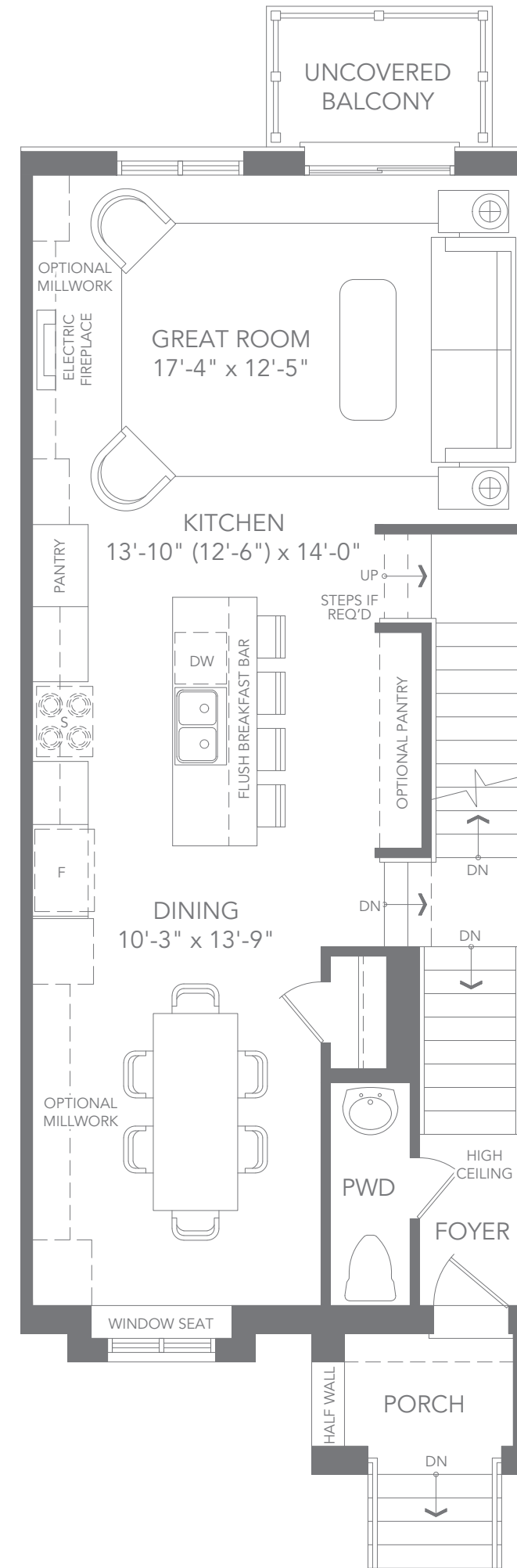
T1 INTERIOR UNIT - ELEV. B2 MAIN FLOOR PLAN
