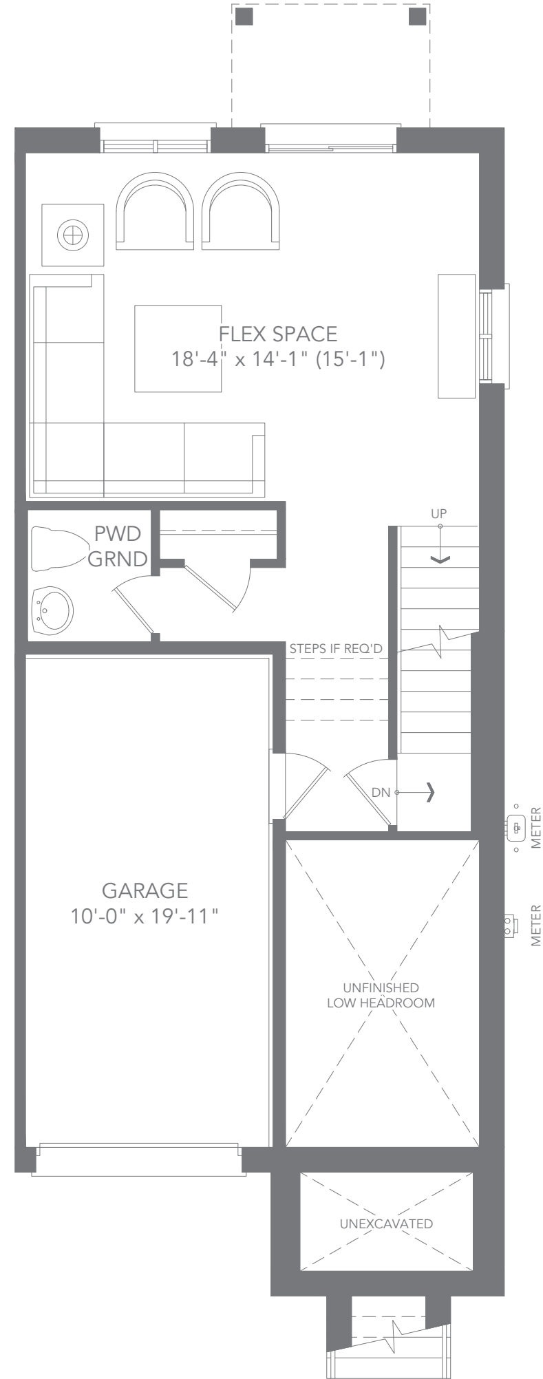
T2 END UNIT - ELEV. A1 GROUND FLOOR PLAN
