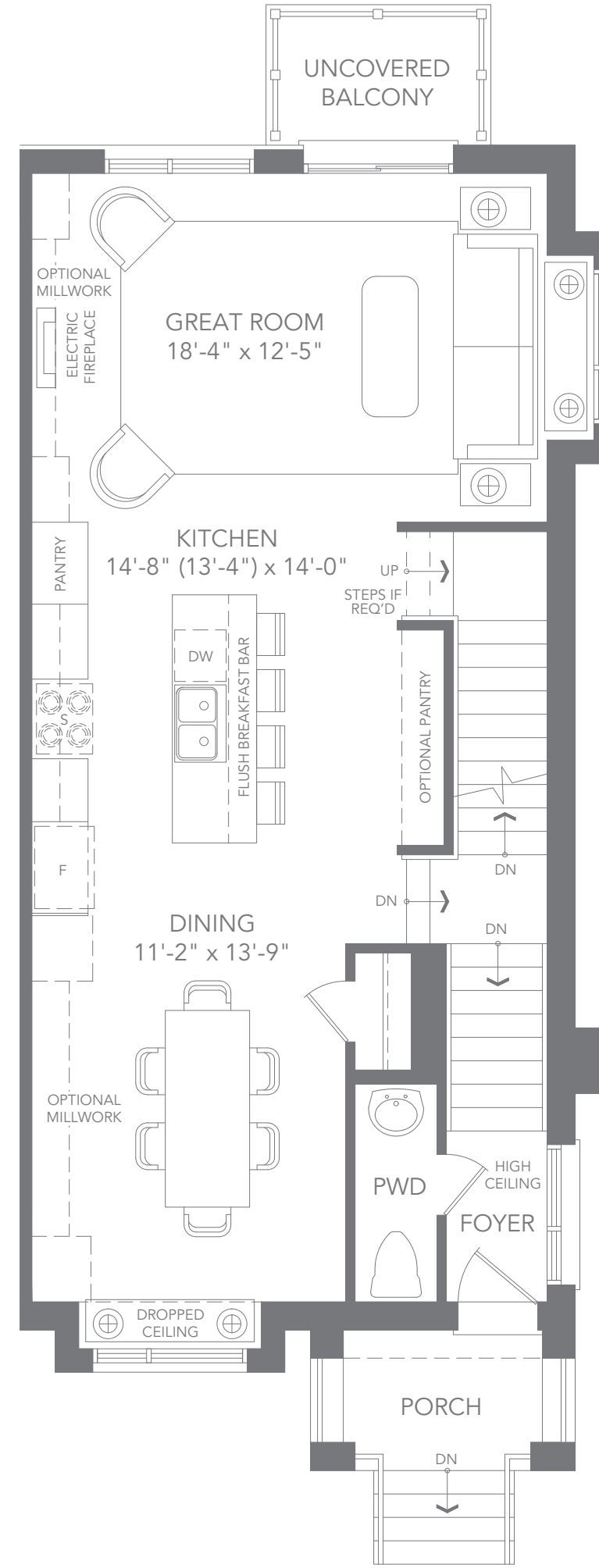
T2 CORNER UNIT - ELEV. C1 MAIN FLOOR PLAN
