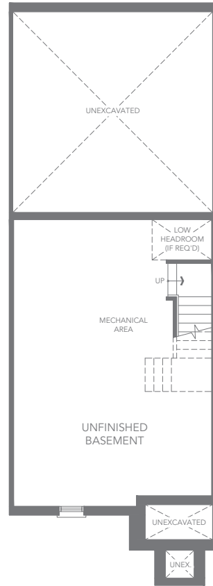
T3 INTERIOR UNIT - ELEV. C1 BASEMENT FLOOR PLAN
