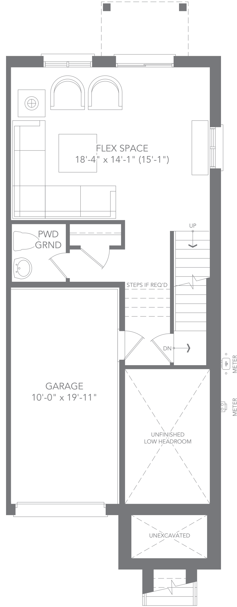
T2 END UNIT - ELEV. B1 GROUND FLOOR PLAN
