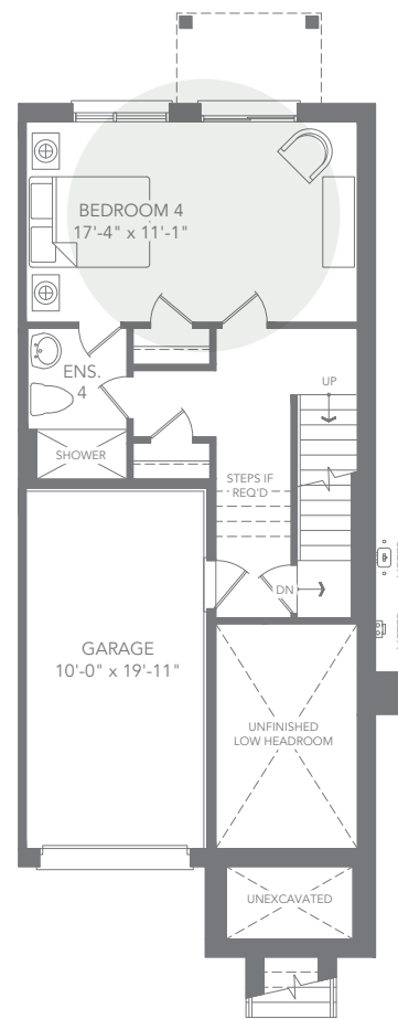
T2 CORNER UNIT - ELEV. C1 OPTIONAL GROUND FLOOR PLAN
