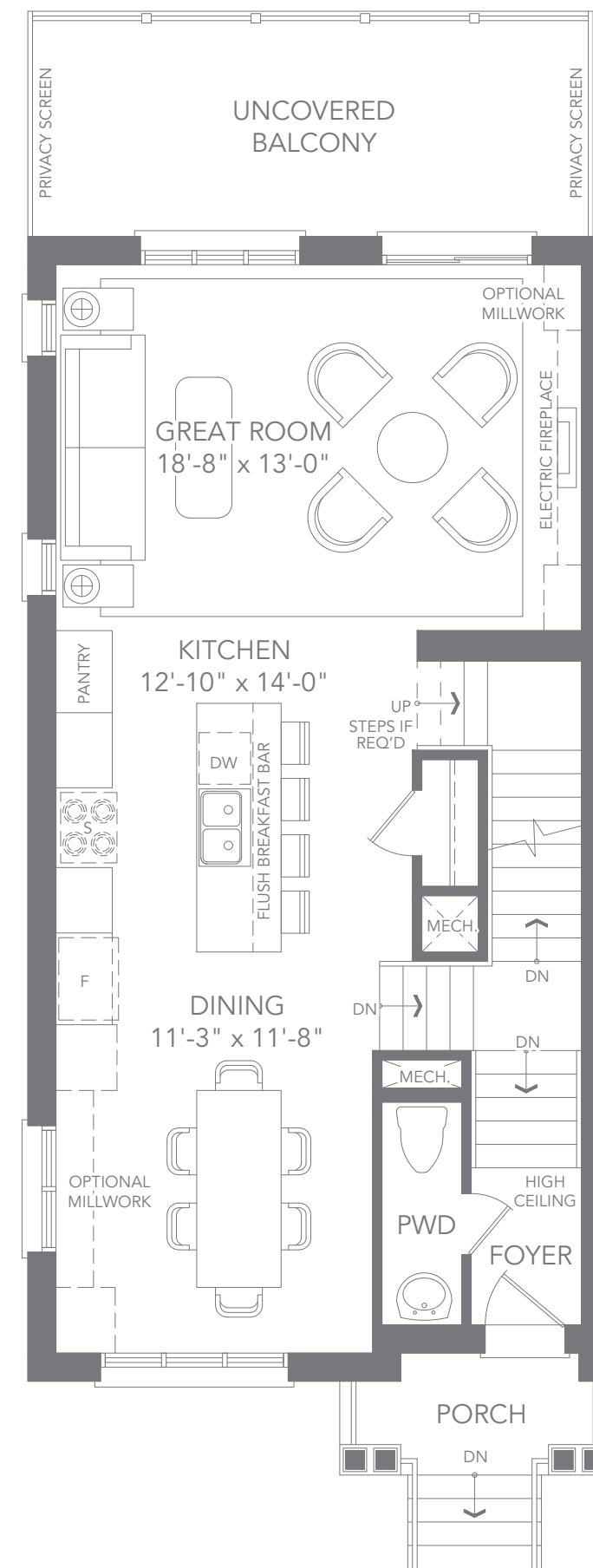
T4 END UNIT - ELEV. A2 MAIN FLOOR PLAN
