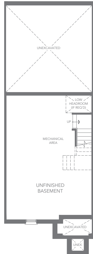
T3 INTERIOR UNIT - ELEV. A2 BASEMENT FLOOR PLAN
