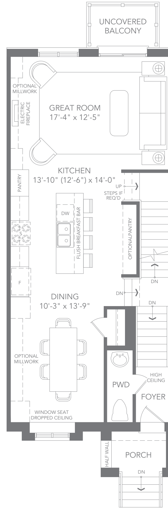
T1 INTERIOR UNIT - ELEV. B1 MAIN FLOOR PLAN
