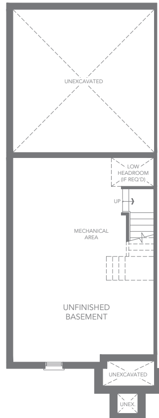
T4 END UNIT - ELEV. B2 BASEMENT FLOOR PLAN
