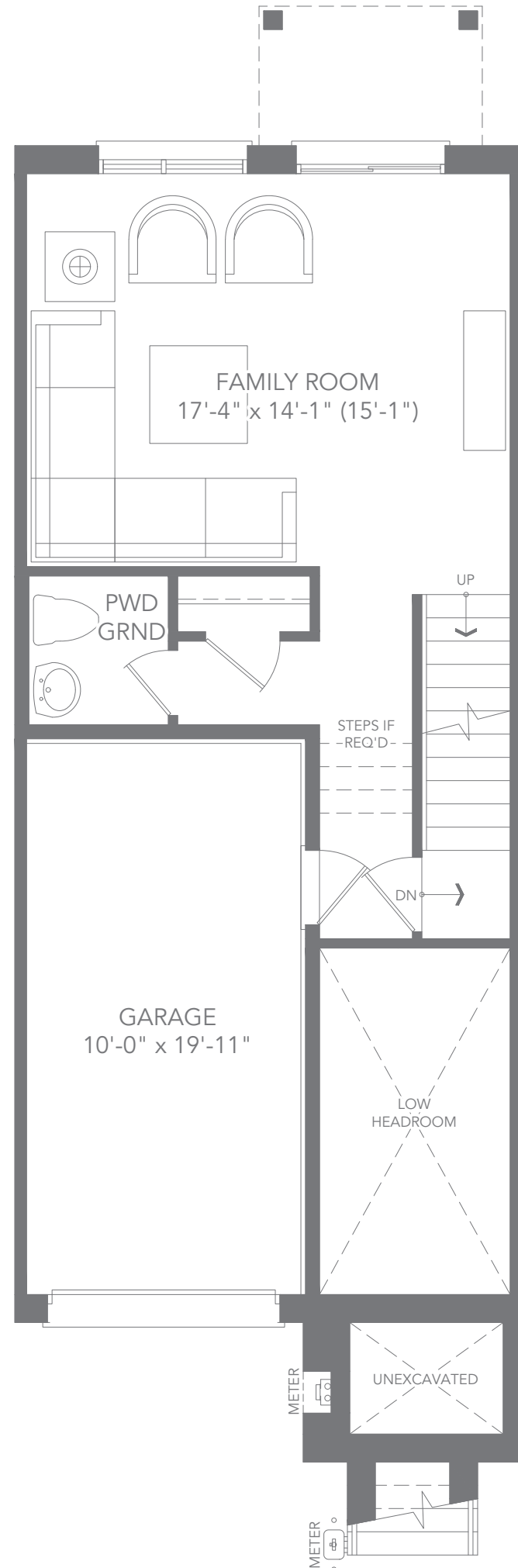
T1 INTERIOR UNIT - ELEV. C4 GROUND FLOOR PLAN
