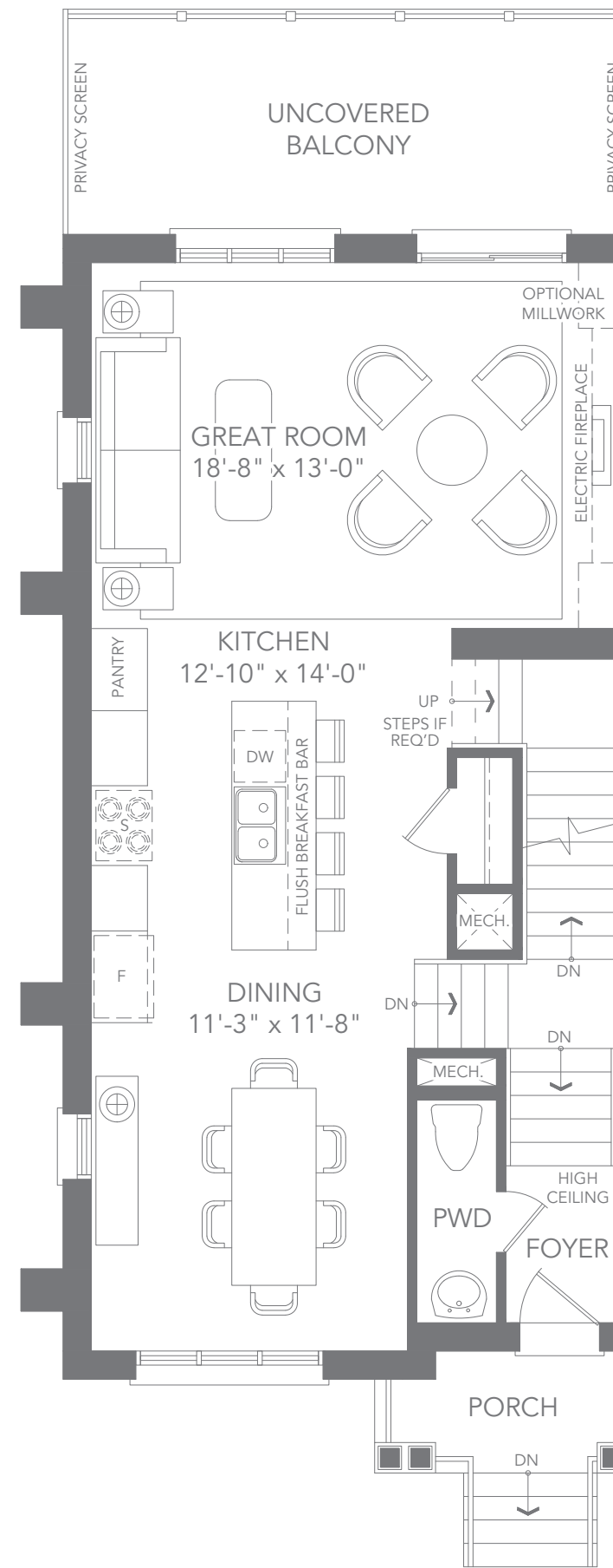
T5 CORNER UNIT - ELEV. A1 MAIN FLOOR PLAN
