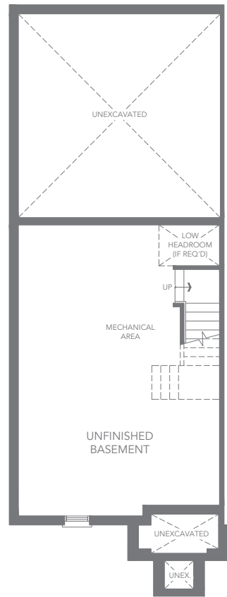
T4 END UNIT - ELEV. A2 BASEMENT FLOOR PLAN
