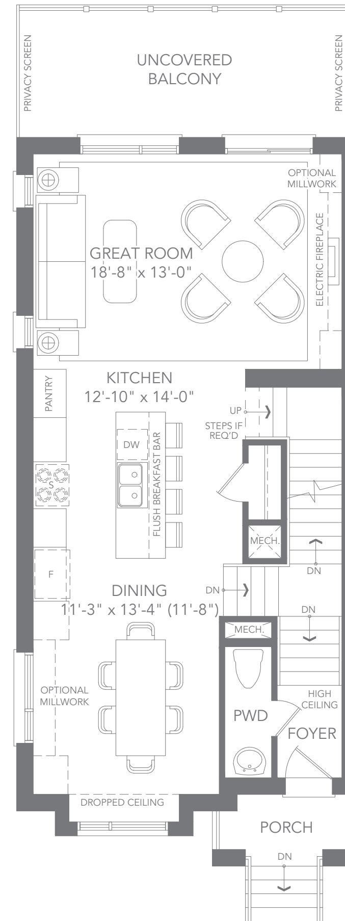
T4 END UNIT - ELEV. C1 MAIN FLOOR PLAN
