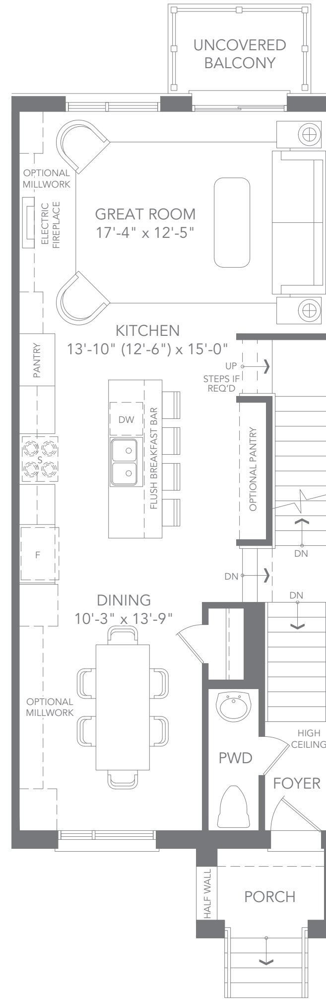
T1 INTERIOR UNIT - ELEV. C4 MAIN FLOOR PLAN
