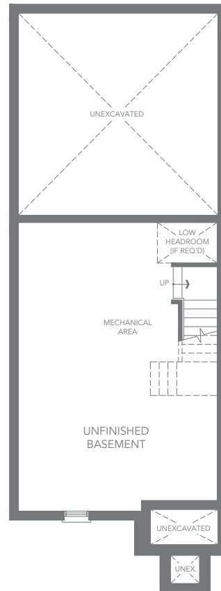
T5 CORNER UNIT - ELEV. C1 BASEMENT FLOOR PLAN
