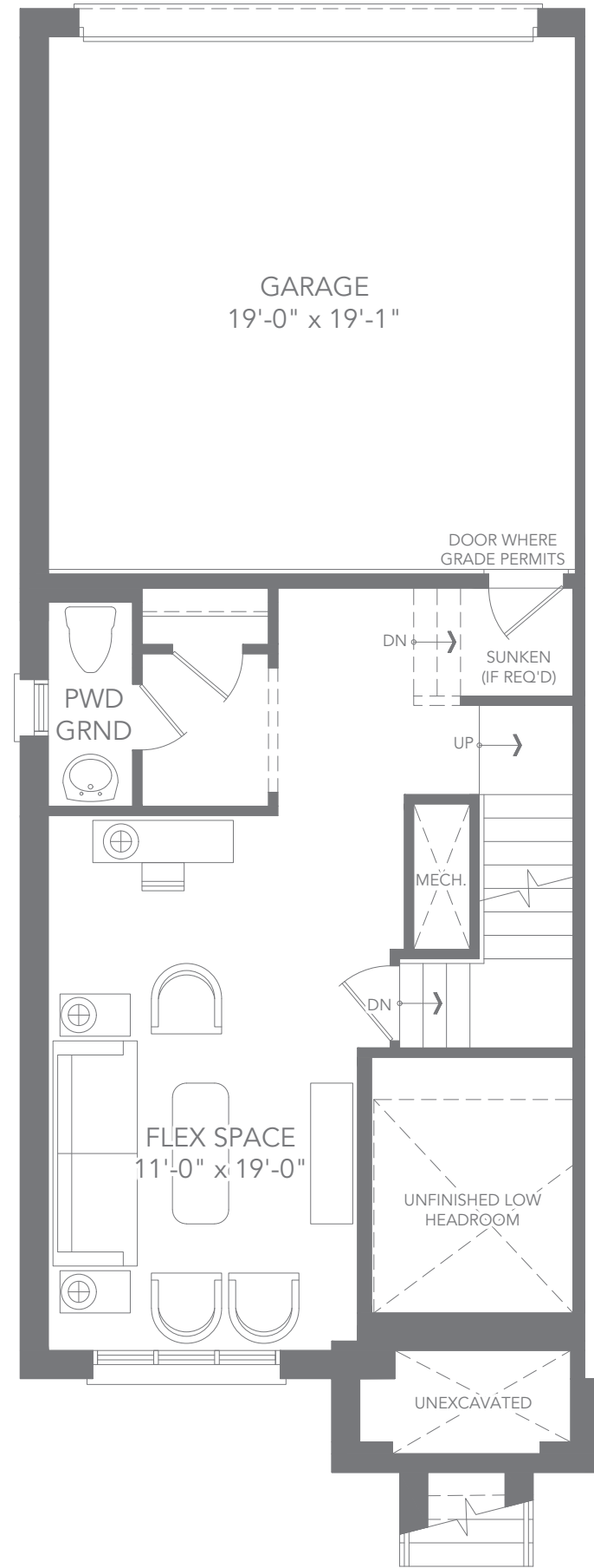
T4 END UNIT - ELEV. A1 GROUND FLOOR PLAN
