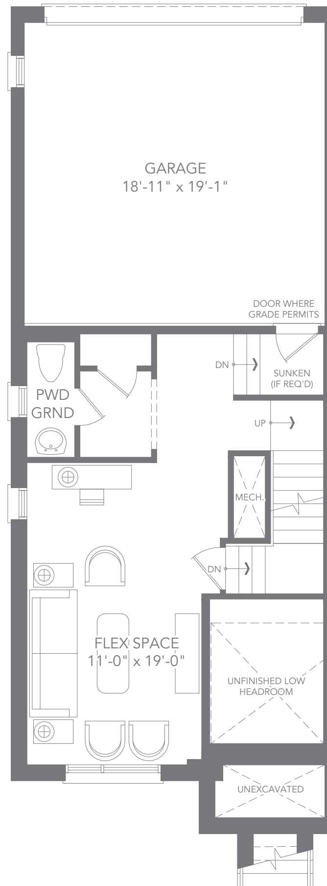
T5 CORNER UNIT - ELEV. C1 GROUND FLOOR PLAN
