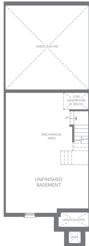
T3 INTERIOR UNIT - ELEV. B1 BASEMENT FLOOR PLAN
