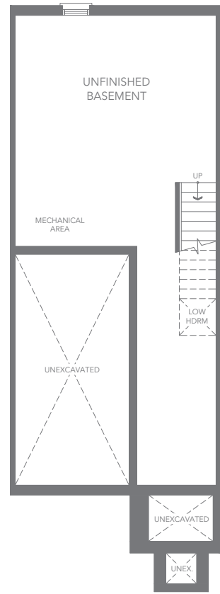
T1 INTERIOR UNIT - ELEV. A1 BASEMENT FLOOR PLAN
