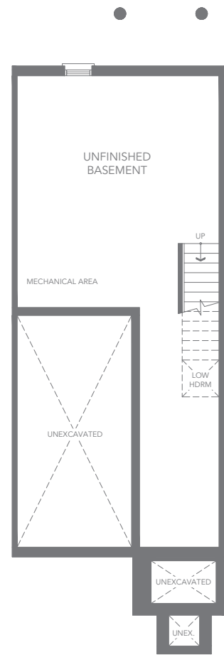
T1 INTERIOR UNIT - ELEV. A3 BASEMENT FLOOR PLAN
