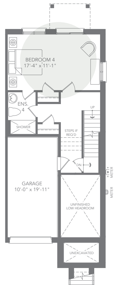
T2 END UNIT - ELEV. B1 OPTIONAL GROUND FLOOR PLAN
