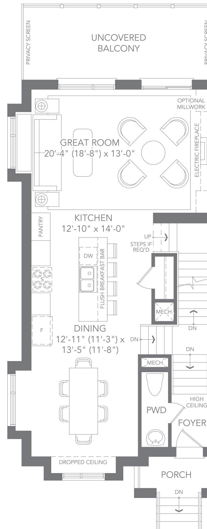
T5 CORNER UNIT - ELEV. C1 MAIN FLOOR PLAN
