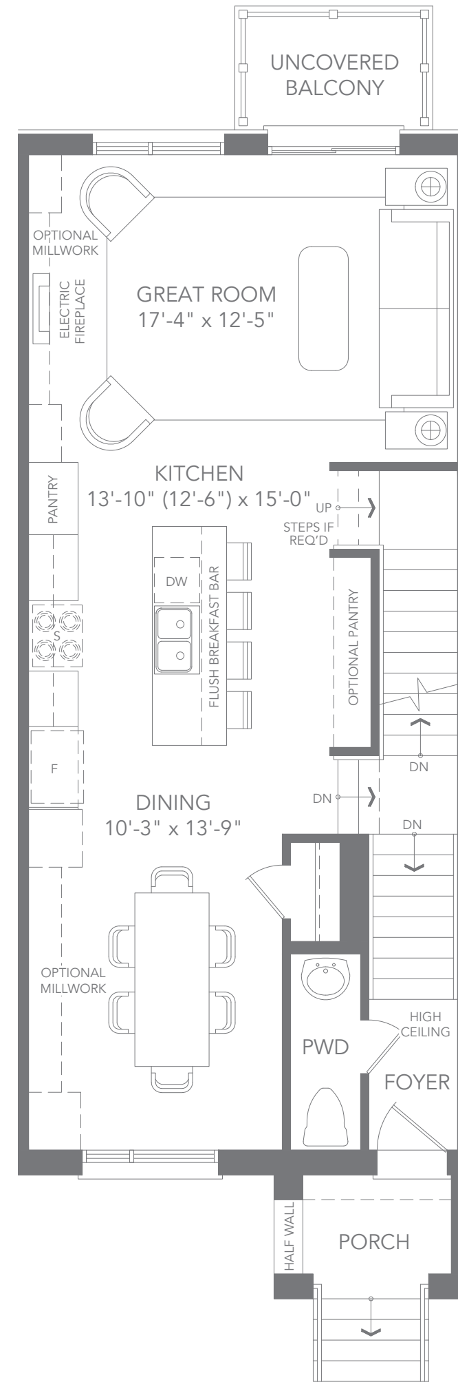
T1 INTERIOR UNIT - ELEV. C2 MAIN FLOOR PLAN
