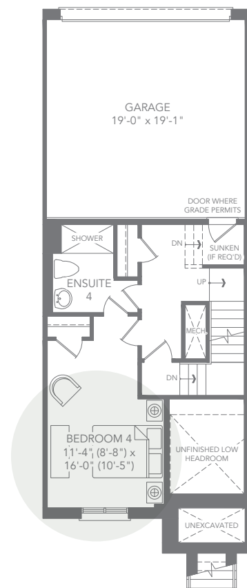
T3 INTERIOR UNIT - ELEV. B1 OPTIONAL GROUND FLOOR PLAN
