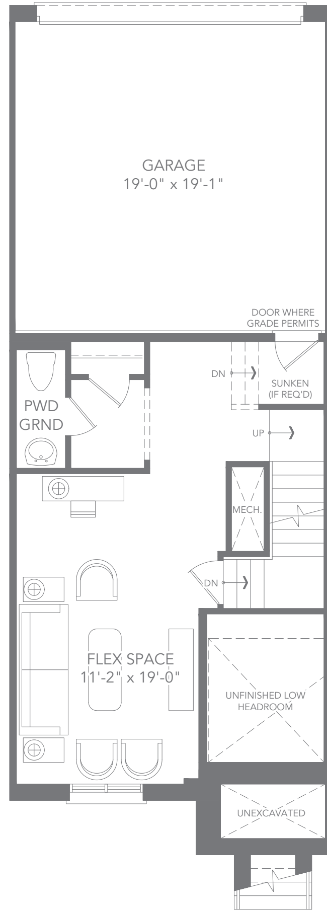
T3 INTERIOR UNIT - ELEV. B1 GROUND FLOOR PLAN
