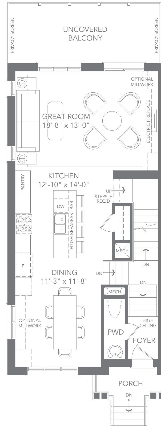
T4 END UNIT - ELEV. A1 MAIN FLOOR PLAN
