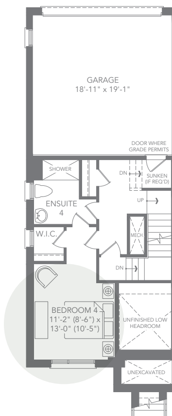
T5 CORNER UNIT - ELEV. C1 OPTIONAL GROUND FLOOR PLAN
