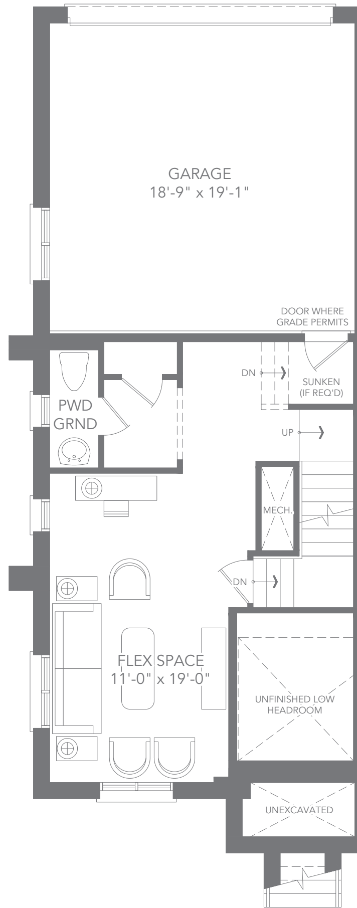
T5 CORNER UNIT - ELEV. B2 GROUND FLOOR PLAN
