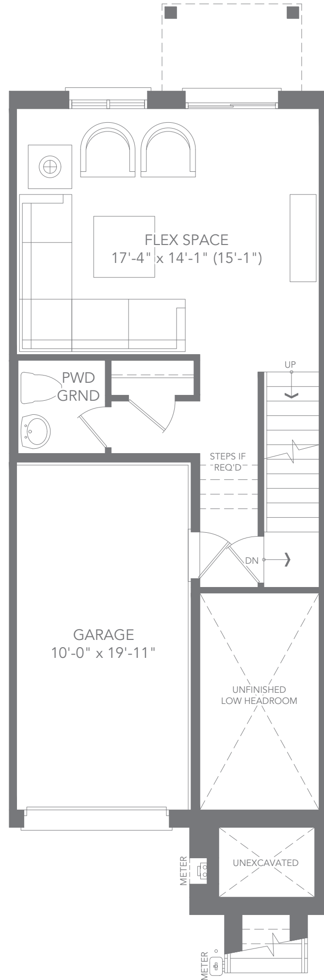
T1 INTERIOR UNIT - ELEV. B1 GROUND FLOOR PLAN
