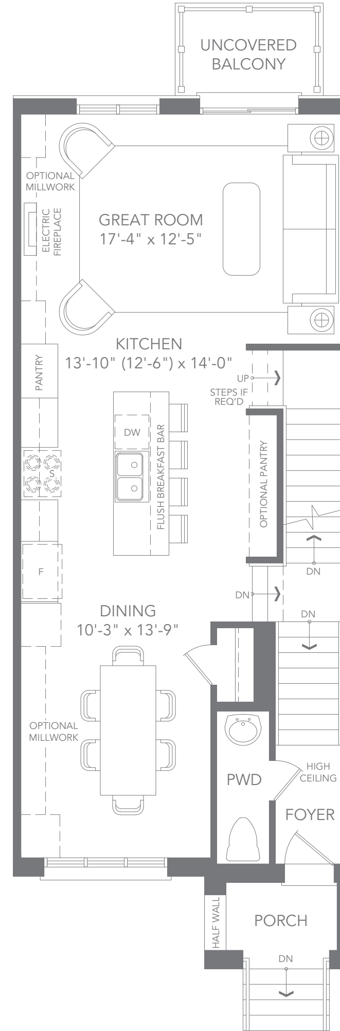
T1 INTERIOR UNIT - ELEV. A3 MAIN FLOOR PLAN
