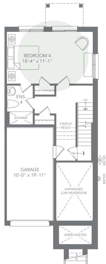
T2 END UNIT - ELEV. C1 OPTIONAL GROUND FLOOR PLAN
