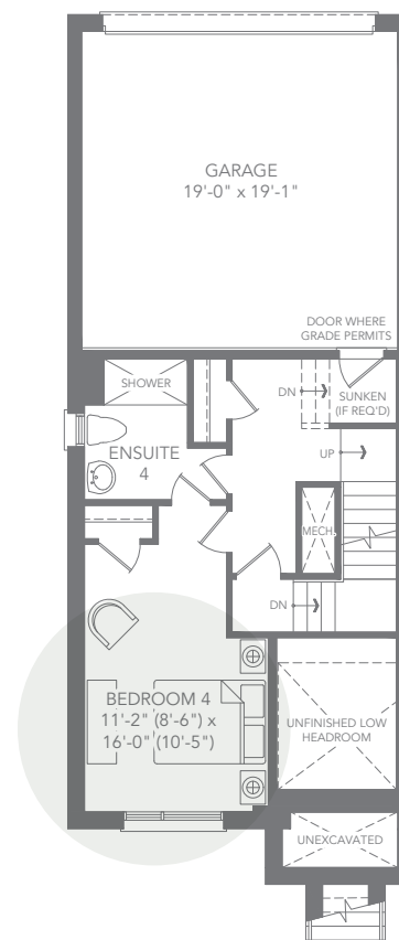
T4 END UNIT - ELEV. C1 OPTIONAL GROUND FLOOR PLAN
