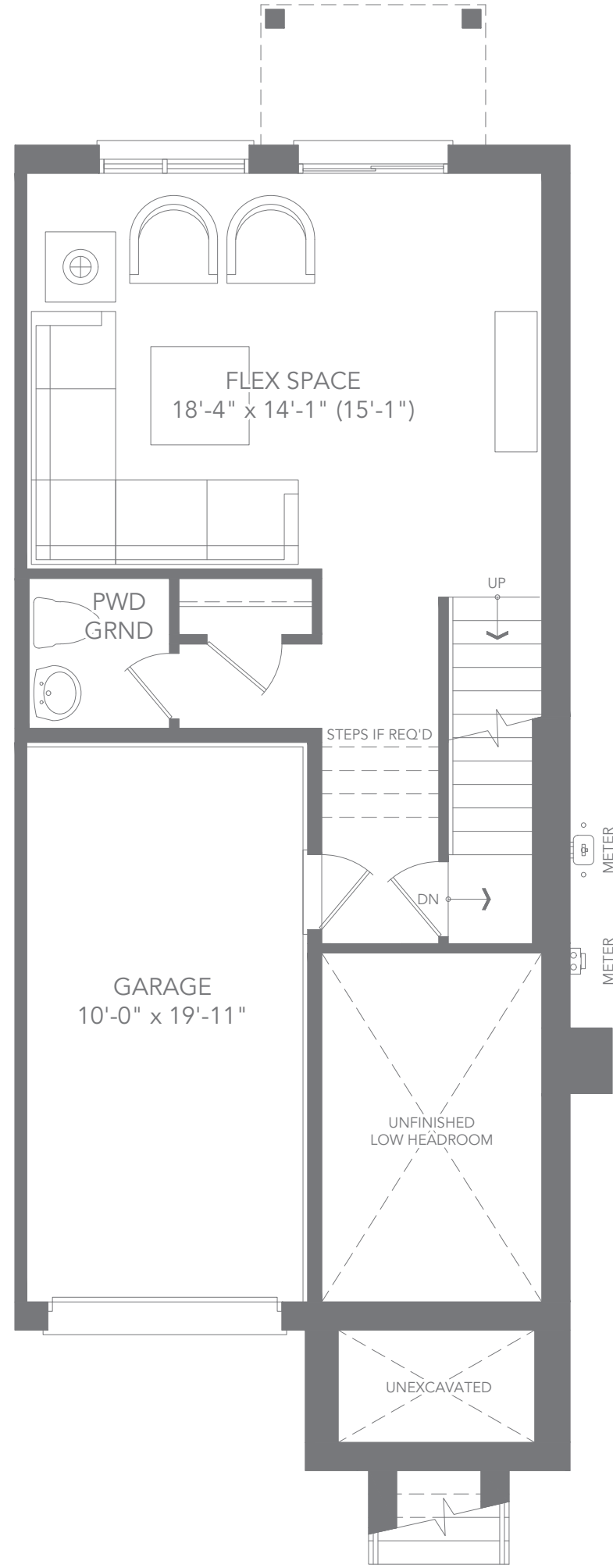
T2 CORNER UNIT - ELEV. C1 GROUND FLOOR PLAN
