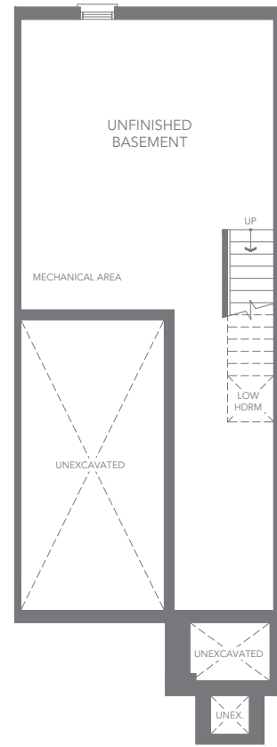
T1 INTERIOR UNIT - ELEV. B2 BASEMENT FLOOR PLAN
