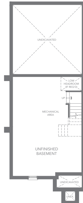
T5 CORNER UNIT - ELEV. B2 BASEMENT FLOOR PLAN
