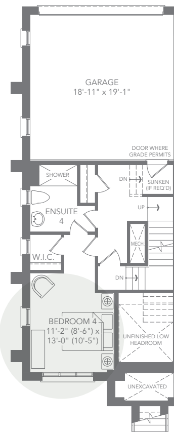
T5 CORNER UNIT - ELEV. A1 OPTIONAL GROUND FLOOR PLAN
