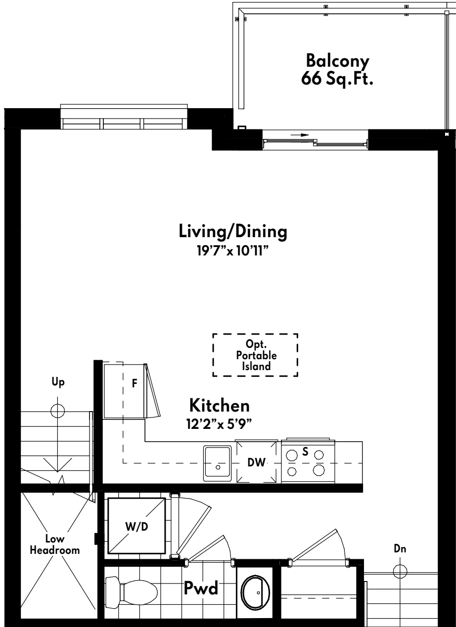
MAIN LEVEL
