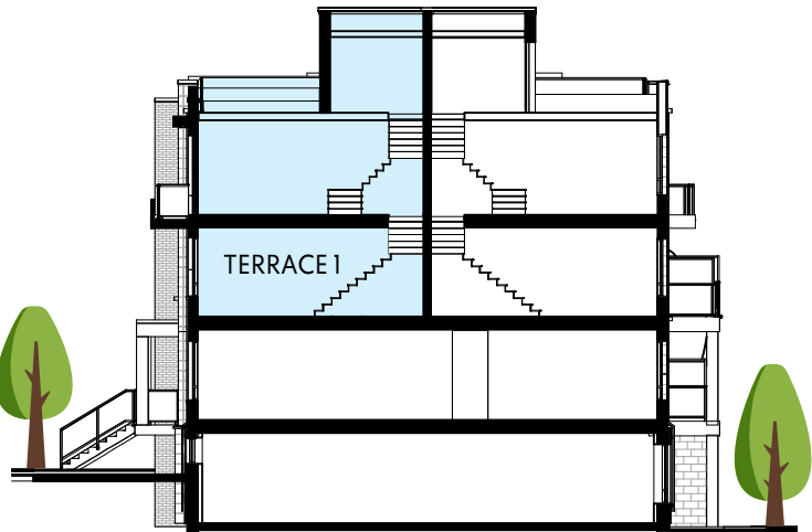
CROSS-SECTION
