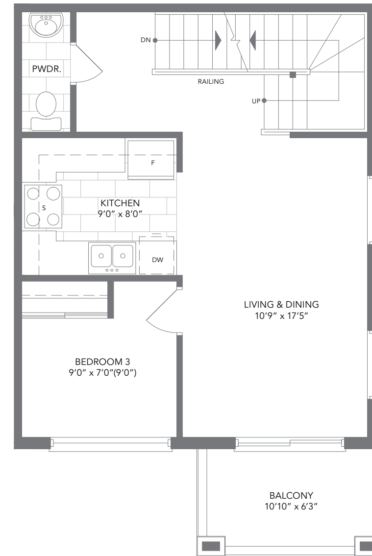
Opt. Second Floor - 3 Bedroom Plan
