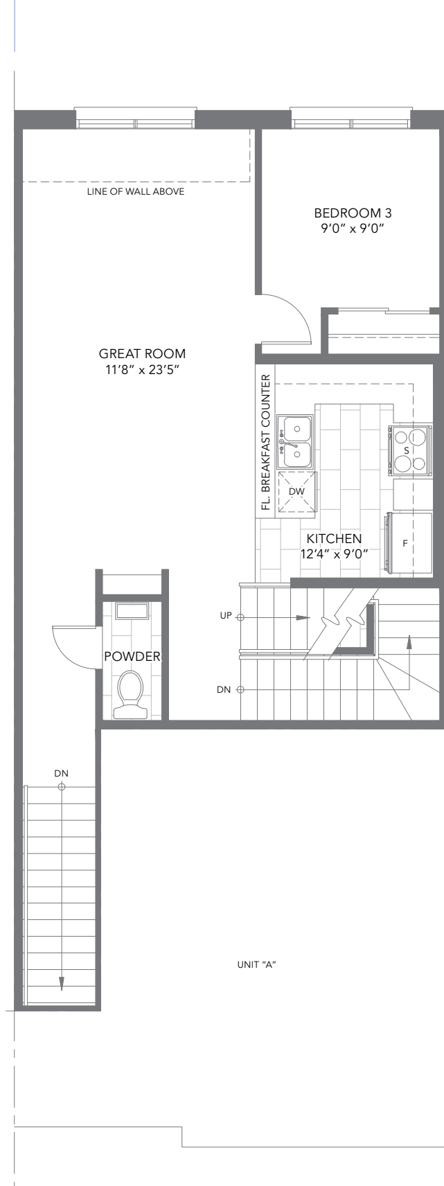
Second Floor Unit B
