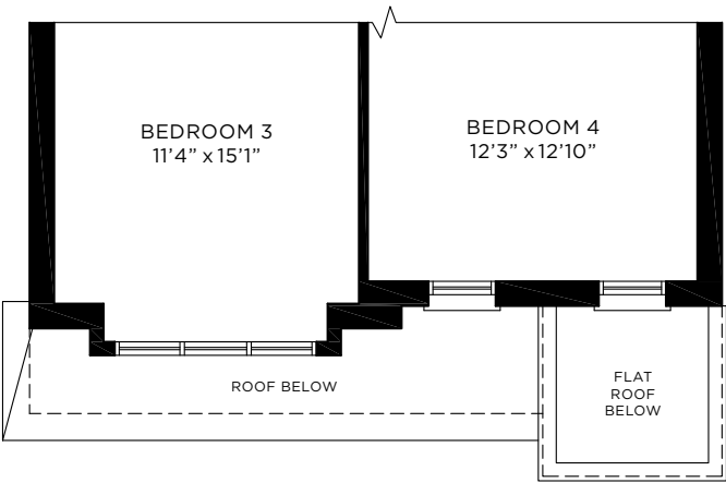
SECOND FLOOR | ELEV. B
