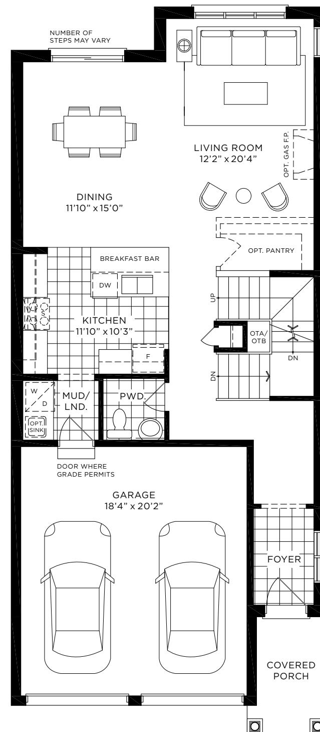
GROUND FLOOR | ELEV. A & B
