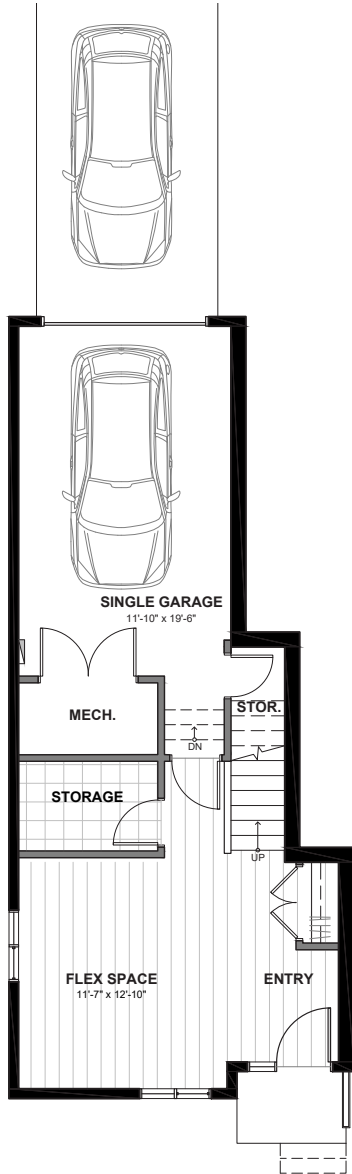
MAIN FLOOR
