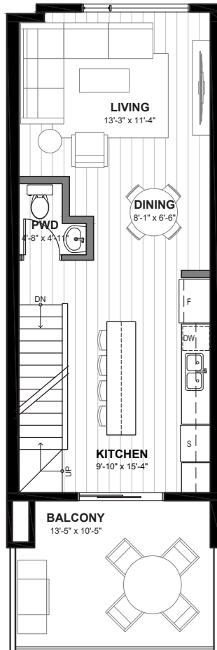
SECOND FLOOR
