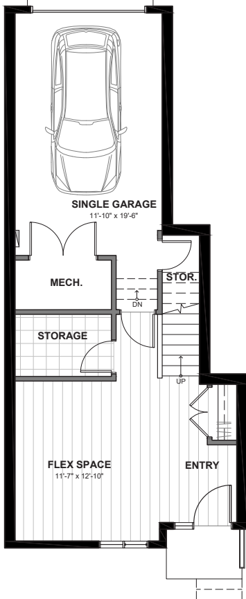
MAIN FLOOR
