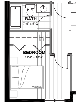
MAIN FLOOR FLEX OPTION 4th Bedroom
