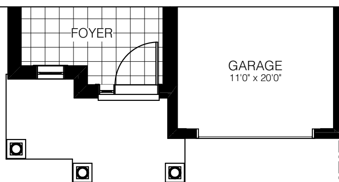
MAIN FLOOR ELEV. B1/B2/B3
