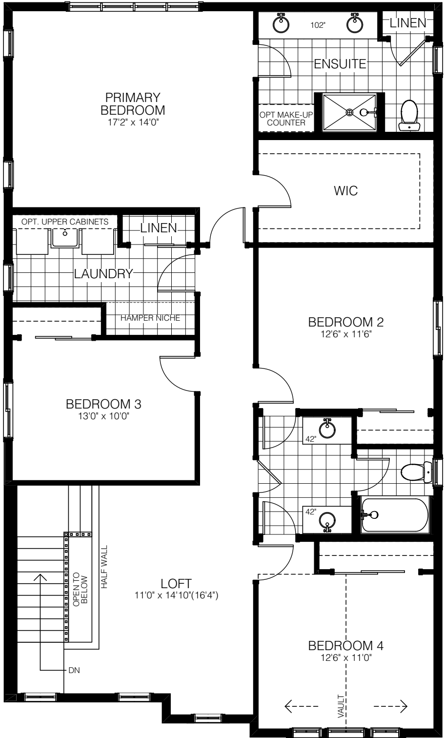
SECOND FLOOR ELEV. A 12 sq.ft. OPEN TO BELOW
