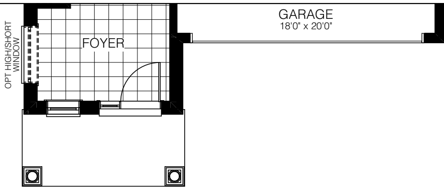
MAIN FLOOR ELEV. B
