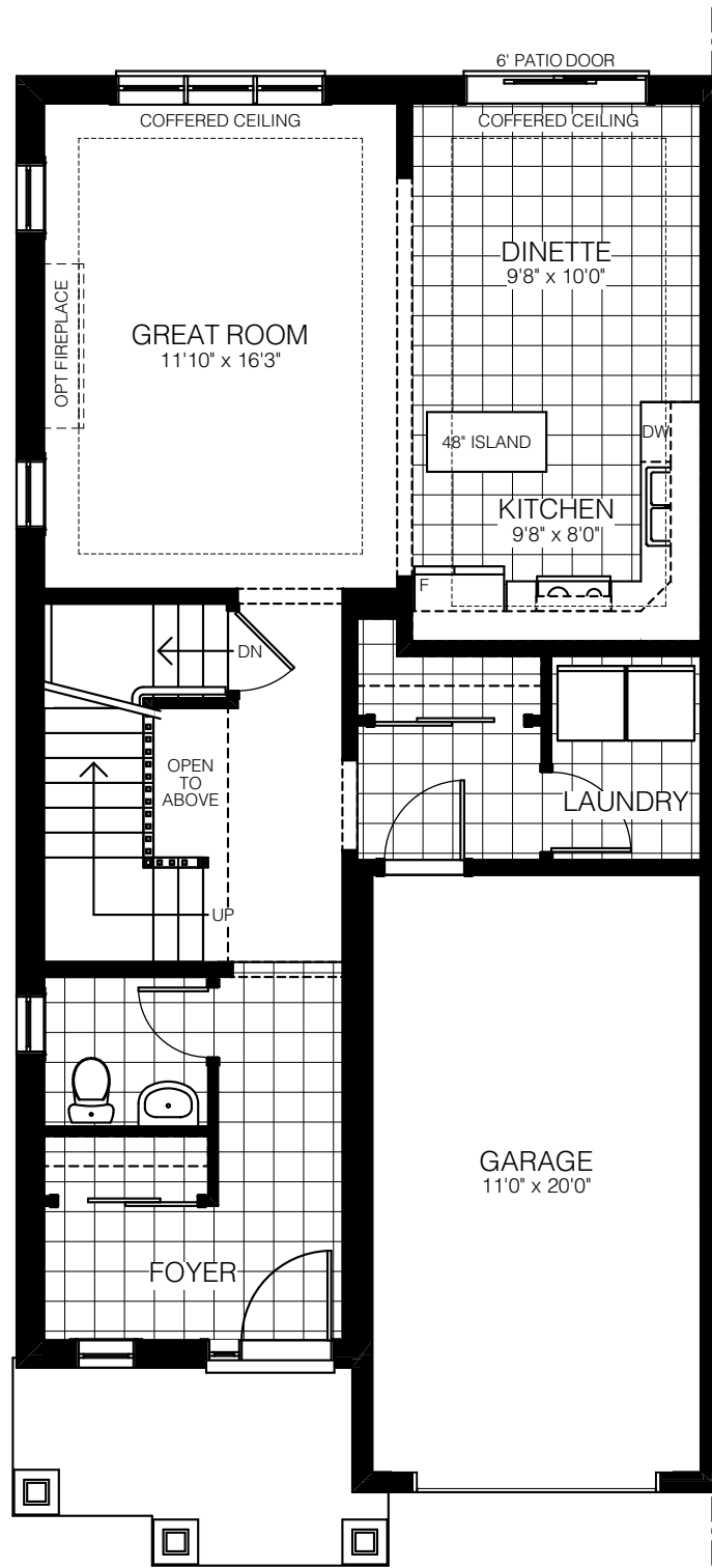
MAIN FLOOR ELEV. A1/A2
