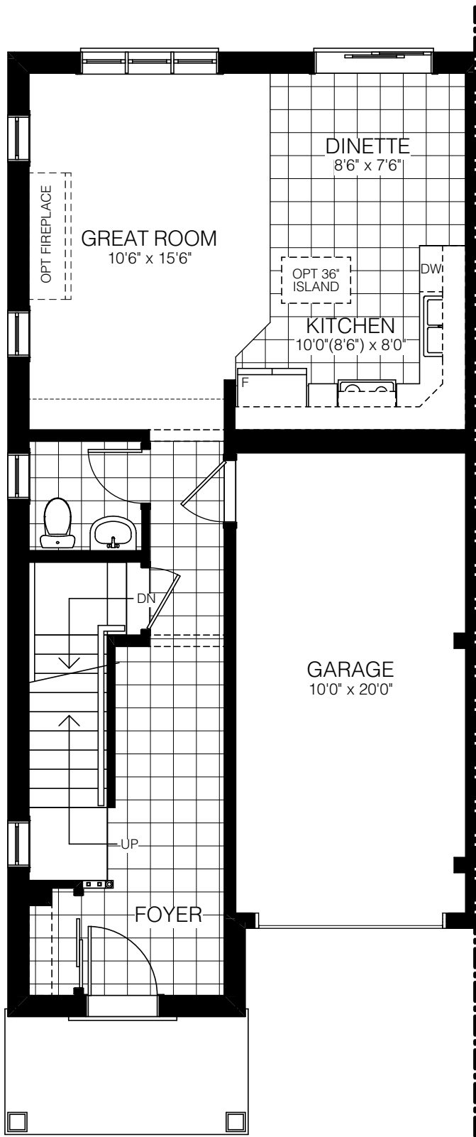
MAIN FLOOR ELEV. A
