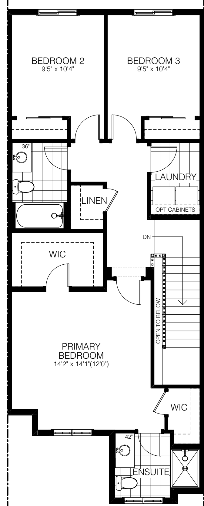
SECOND FLOOR ELEV. A
