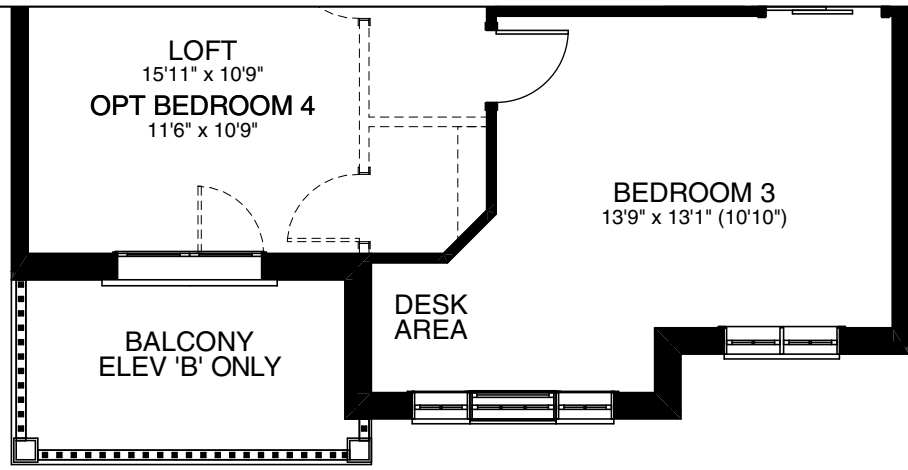
SECOND FLOOR ELEV. B
