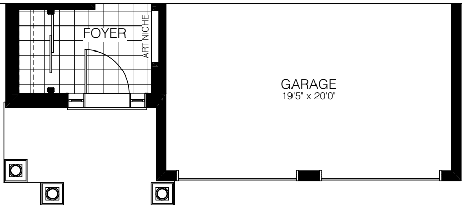
MAIN FLOOR ELEV. B
