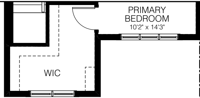
SECOND FLOOR ELEV. B1/B2
