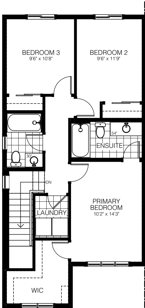
OPTIONAL SECOND FLOOR 3PC BATH UPGRADE
