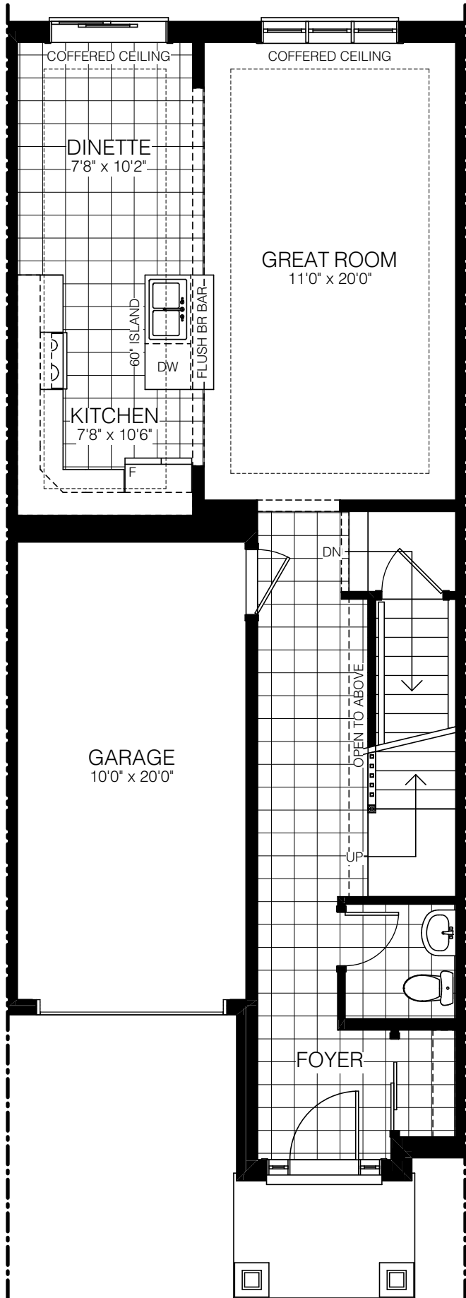
MAIN FLOOR ELEV. A/B
