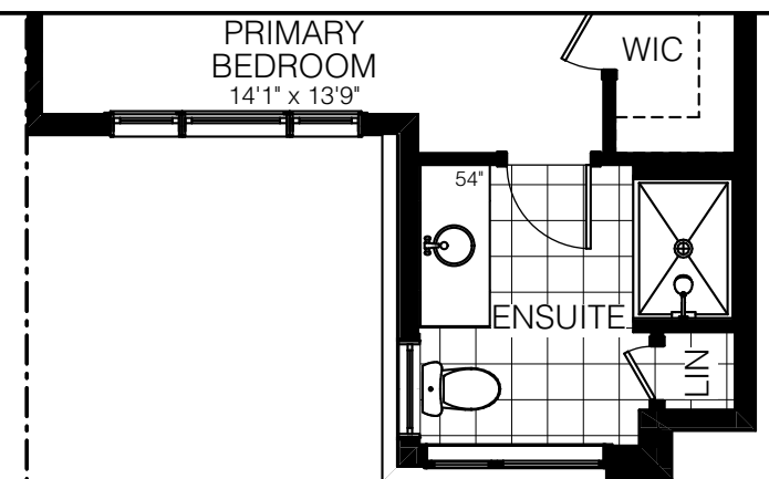
SECOND FLOOR ELEV. M2
