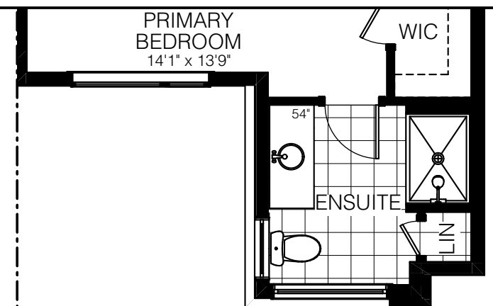
SECOND FLOOR ELEV. M1
