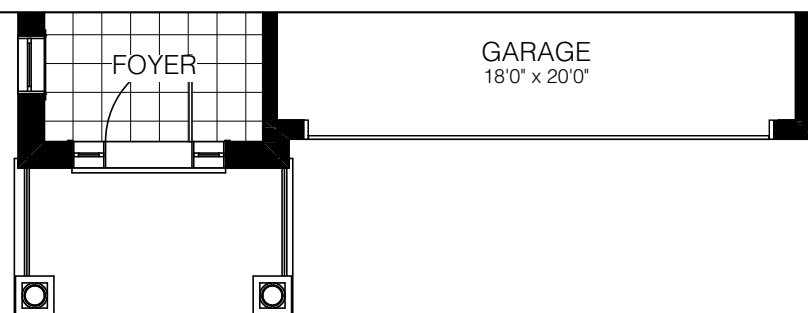
MAIN FLOOR ELEV. B
