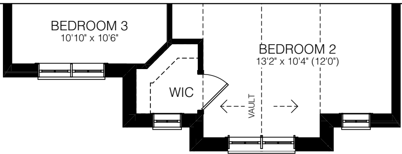
SECOND FLOOR ELEV. B
