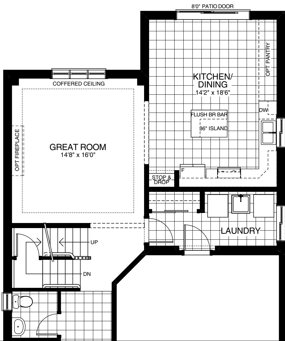
OPTIONAL MAIN FLOOR LAUNDRY BUMPOUT UPGRADE
