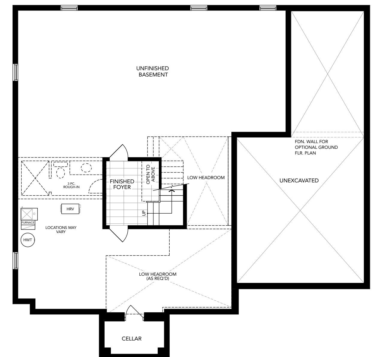
Basement Plan Elevation A
