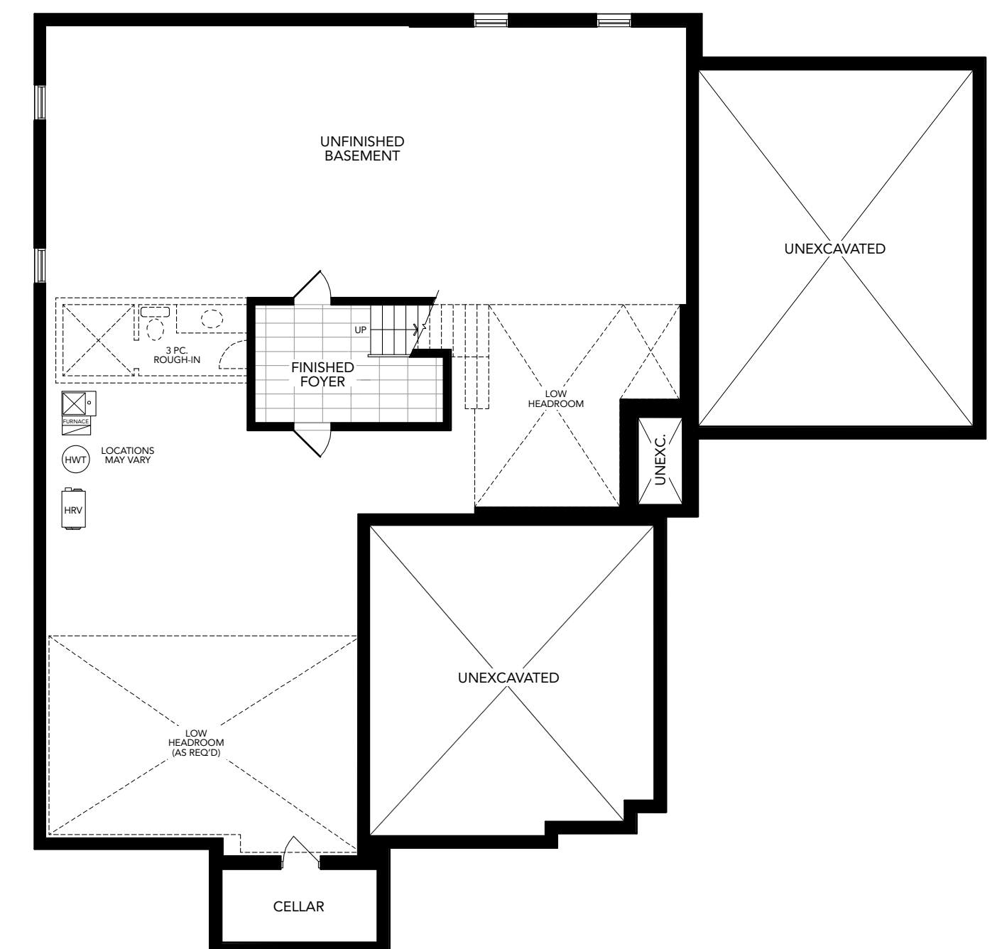
Basement Floor Plan Elevation B
