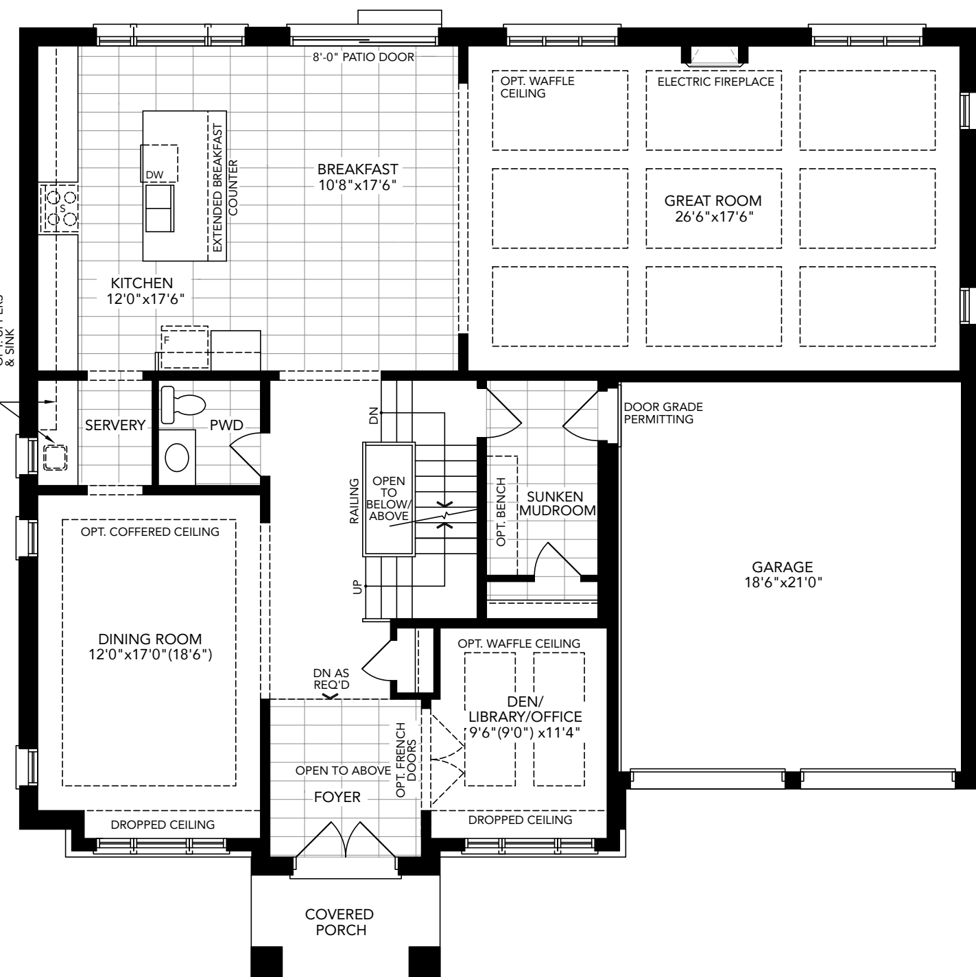
Opt. Ground Floor Plan Elevation A
