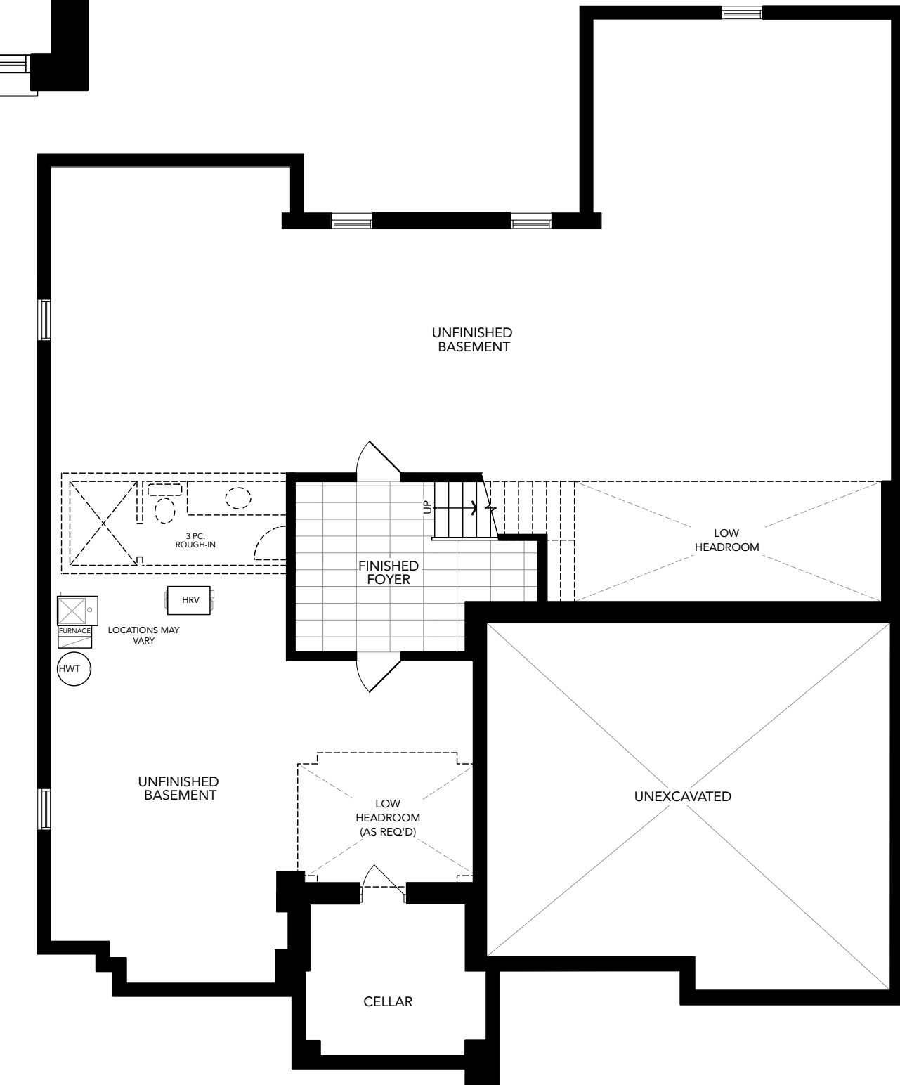
Basement Floor Plan Elevation A
