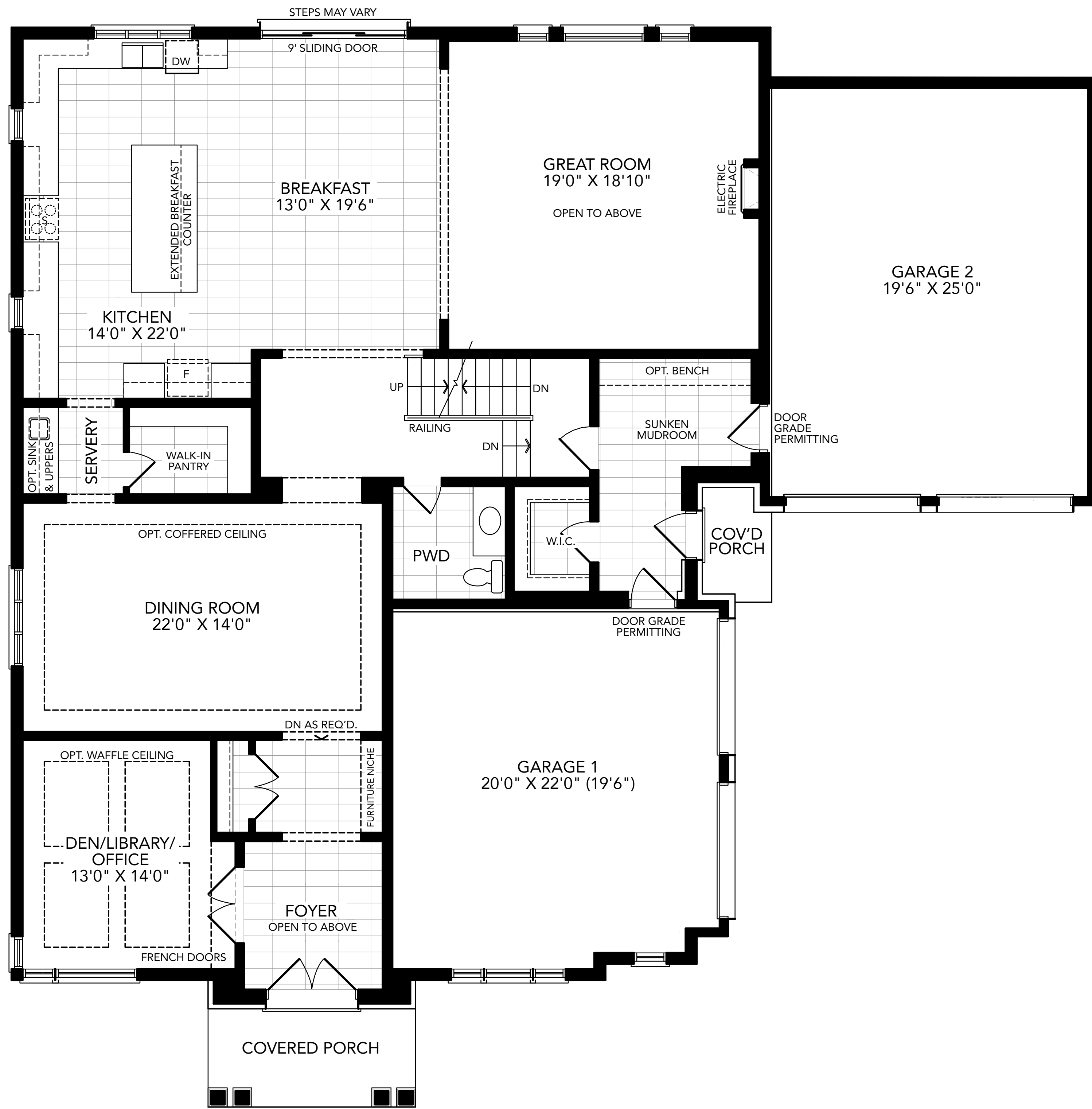
Ground Floor Plan Elevation B
