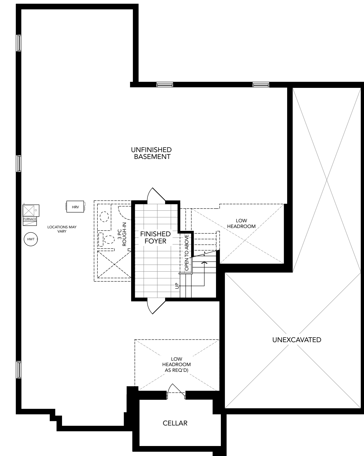
Basement Plan Elevation A
