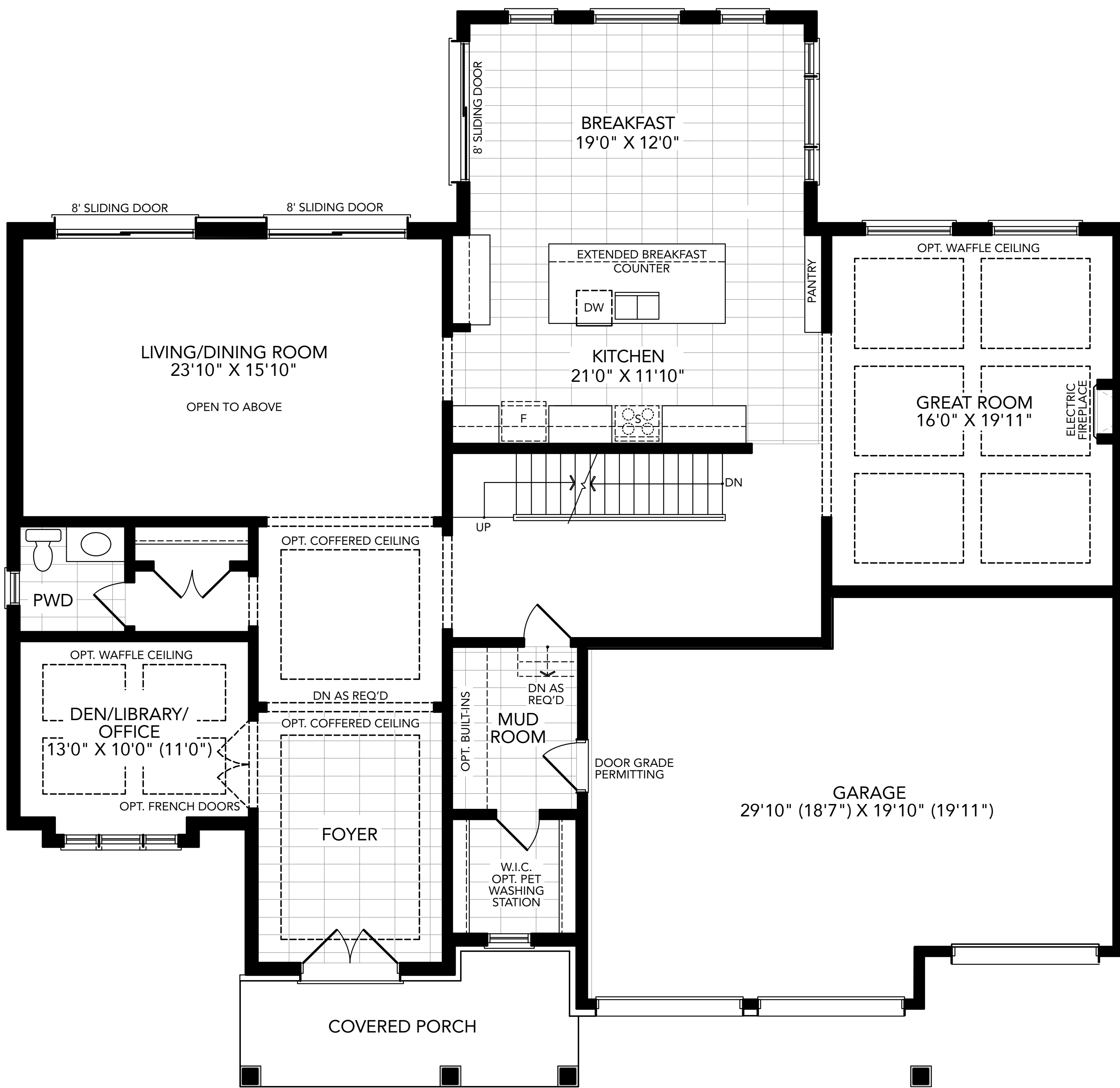
Ground Floor Plan Elevation B
