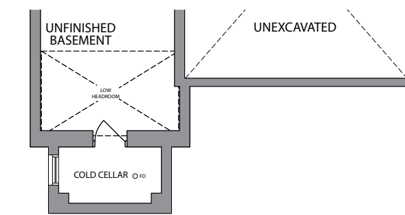
BASEMENT ELEV. C
