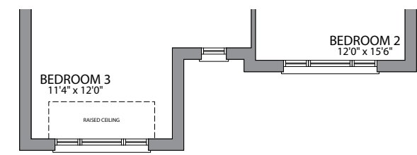
OPT. SECOND FLOOR ELEV. C
