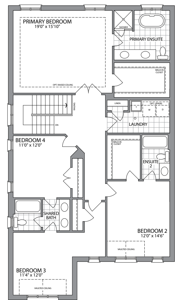
OPT. SECOND FLOOR ELEV. A
