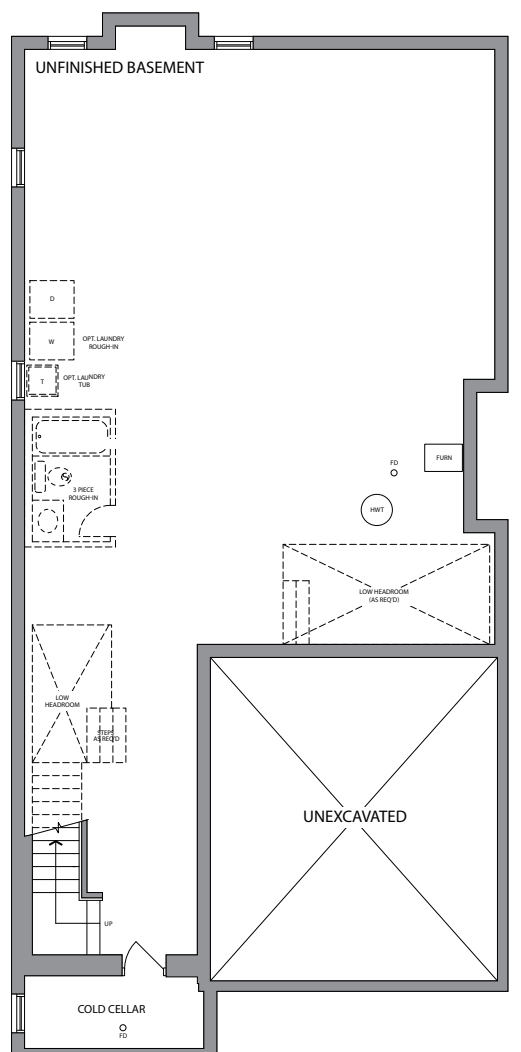
BASEMENT ELEV. A & B
