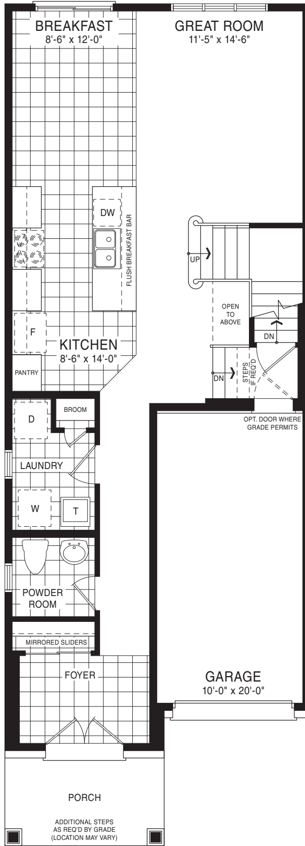
MAIN FLOOR PLAN STYLE A1
