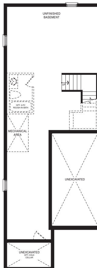
BASEMENT PLAN STYLE A1
