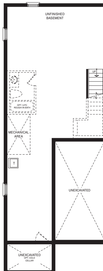
BASEMENT PLAN STYLE A1
