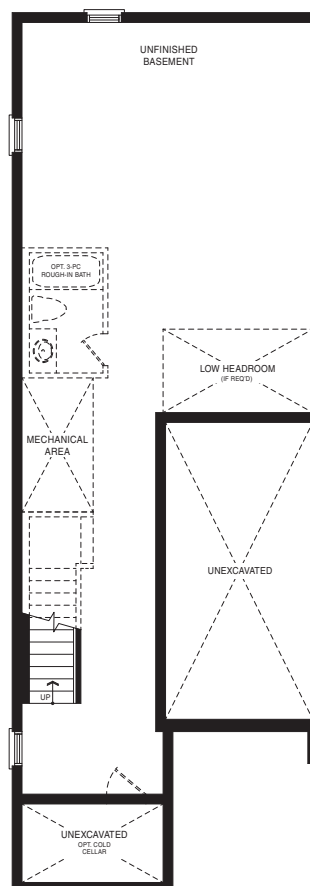
BASEMENT PLAN STYLE A1
