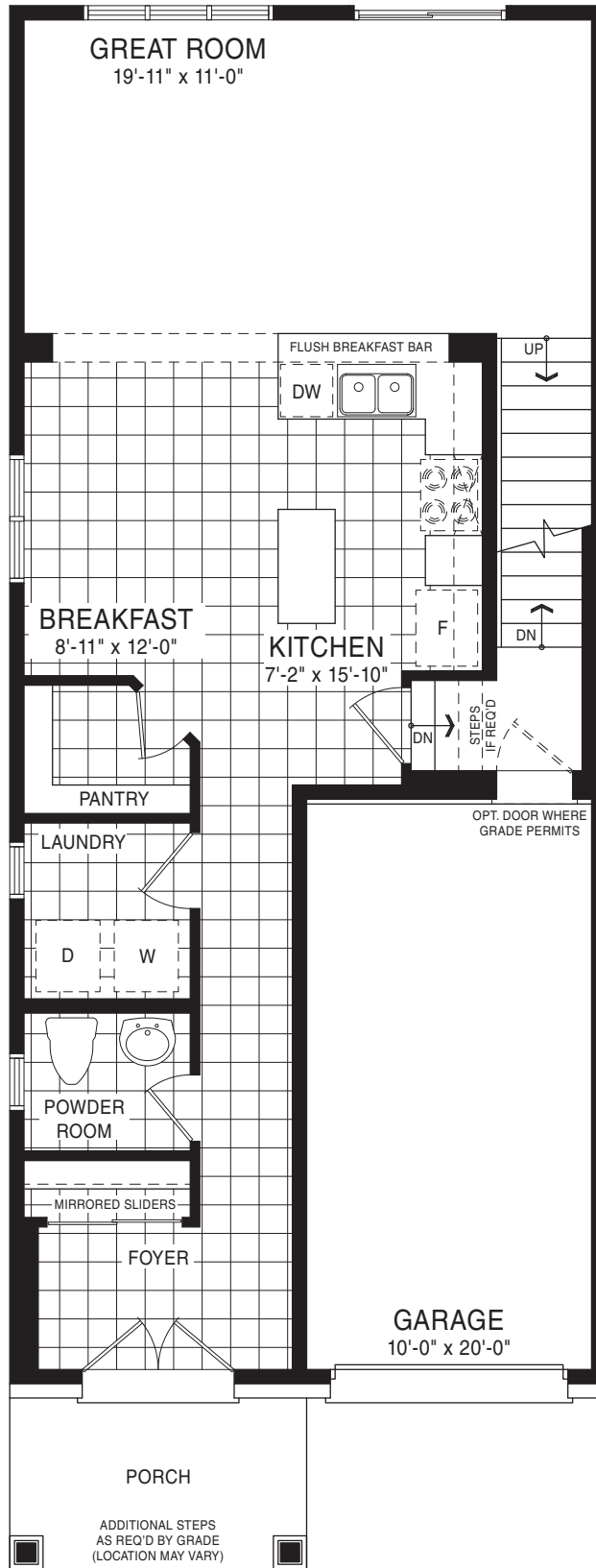
MAIN FLOOR PLAN STYLE A1
