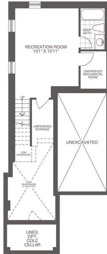
345 sf OF OPT. FINISHED BASEMENT ELEVATION A 1872 sf
