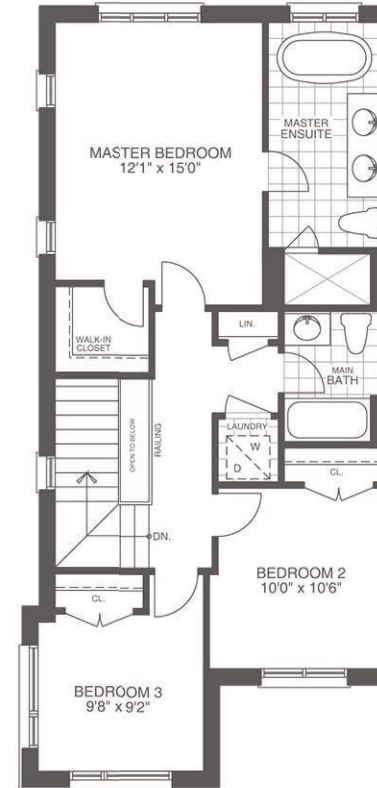
SECOND FLOOR PLAN ELEVATION A 1527 sf
