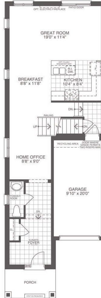
GROUND FLOOR PLAN ELEVATION A 1933 sf
