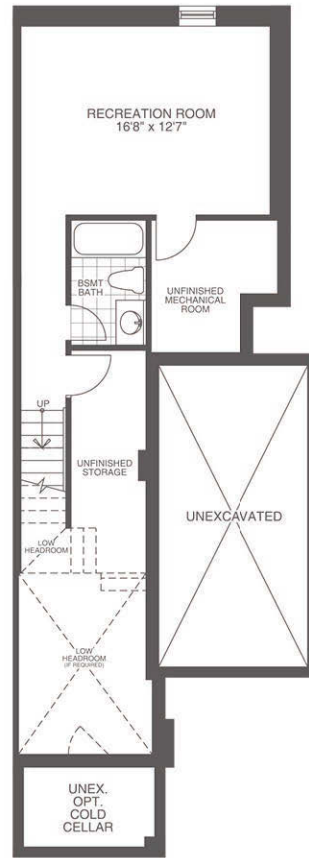
358 sf OF OPT. FINISHED BASEMENT ELEVATION A & A1 1960 sf
