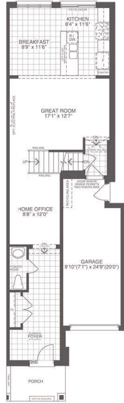
GROUND FLOOR PLAN ELEVATION A 1966 sf
