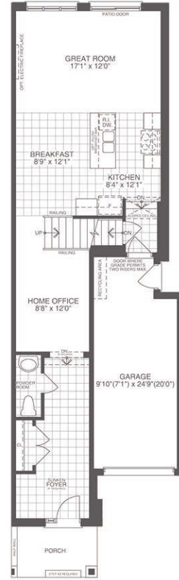
ALT. GROUND FLOOR PLAN ELEVATION A 1966 sf
