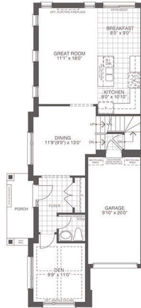
GROUND FLOOR PLAN ELEVATION A 1986 sf
