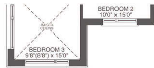
SECOND FLOOR PLAN ELEVATION B 1956 sf
