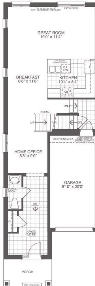
GROUND FLOOR PLAN ELEVATION A 1933 sf
