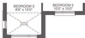
SECOND FLOOR PLAN ELEVATION B 1933 sf
