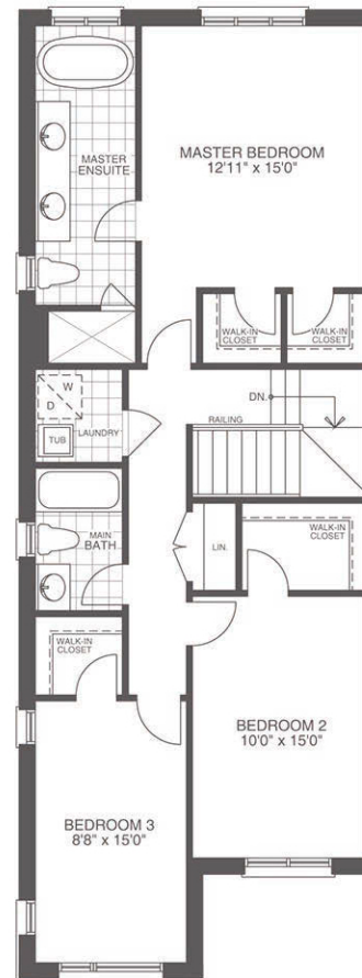
SECOND FLOOR PLAN ELEVATION A 1933 sf
