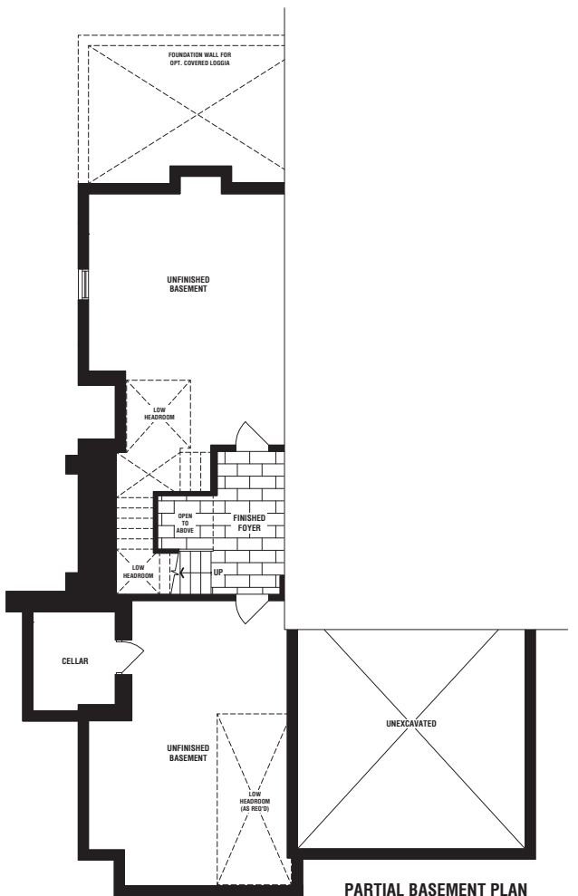
PARTIAL BASEMENT PLAN ELEV. 'C'
