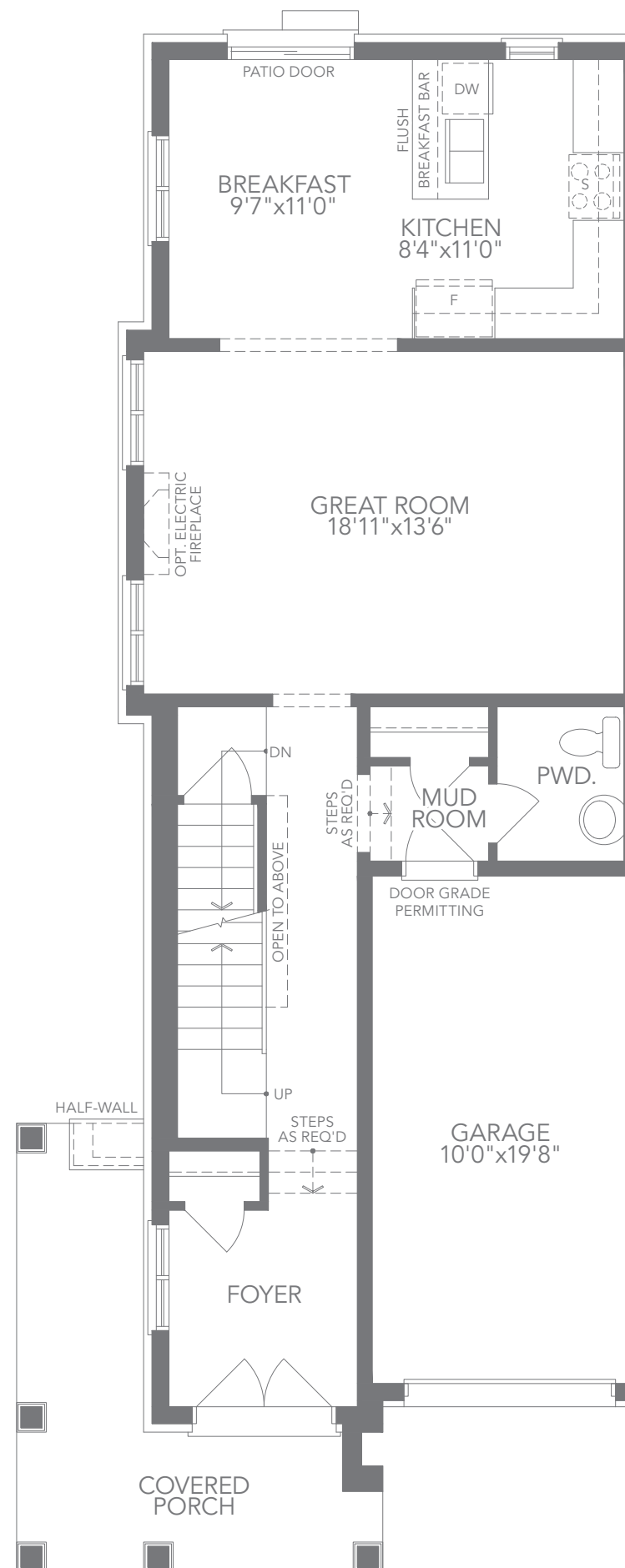
T3 COR - ELEV. A4 GROUND FLOOR PLAN
