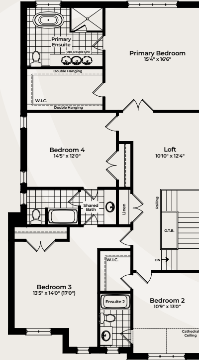
ELEV. A 3,954 SQ.FT.
