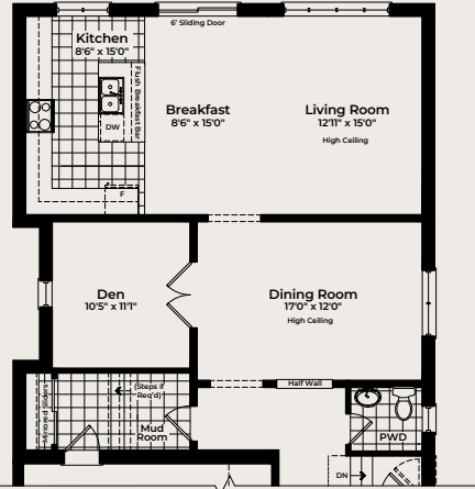
PART. ALT. GROUND FLOOR W/ DEN Elev. A, B & C
