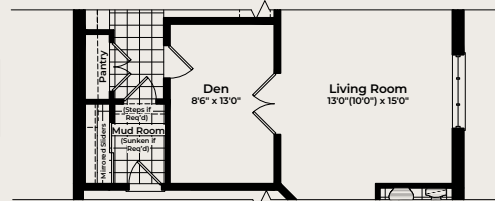
PART. GROUND FLOOR W/ Opt. Den Elev. A, B & C
