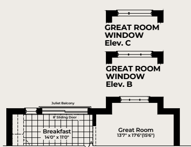
PART. GROUND FLOOR WOB CONDITION Elev. A, B & C
