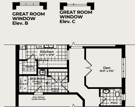
PART. GROUND FLOOR W/ Opt. Den Elev. A, B & C
