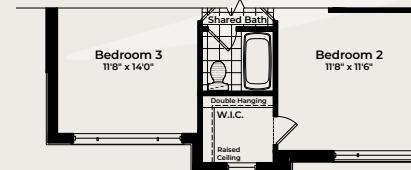
PART. SECOND FLOOR Elev. C
