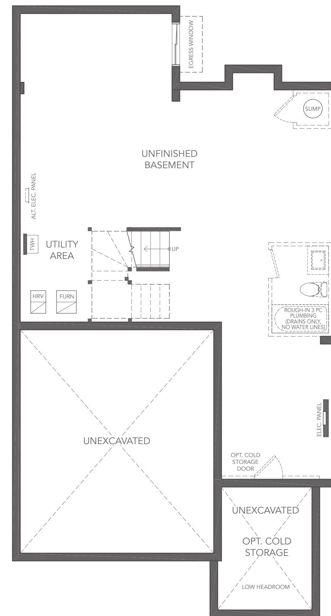
BASEMENT PLAN A
